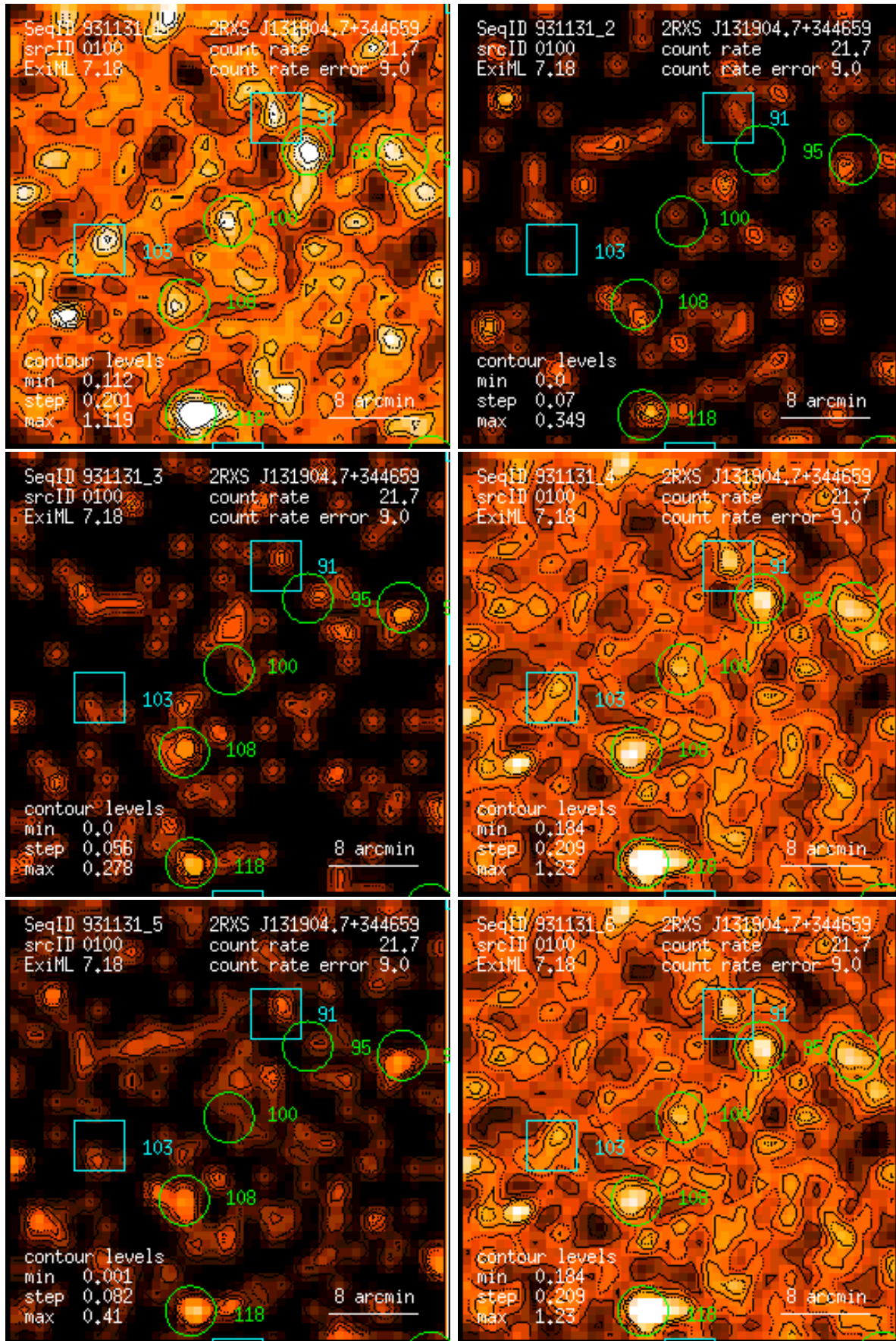
Figure 100: RASS 931131: detection 0100: band rate images, Gaussian filter: (1) PSPC channels 11 – 41, (2) 52 – 90, (3) 91 – 201, (4) 11 – 235, (5) 52 – 201, (6) 11 – 201. Broad band rates in counts/ks. Band rate contour levels in counts/ks/arcmin 2 .
