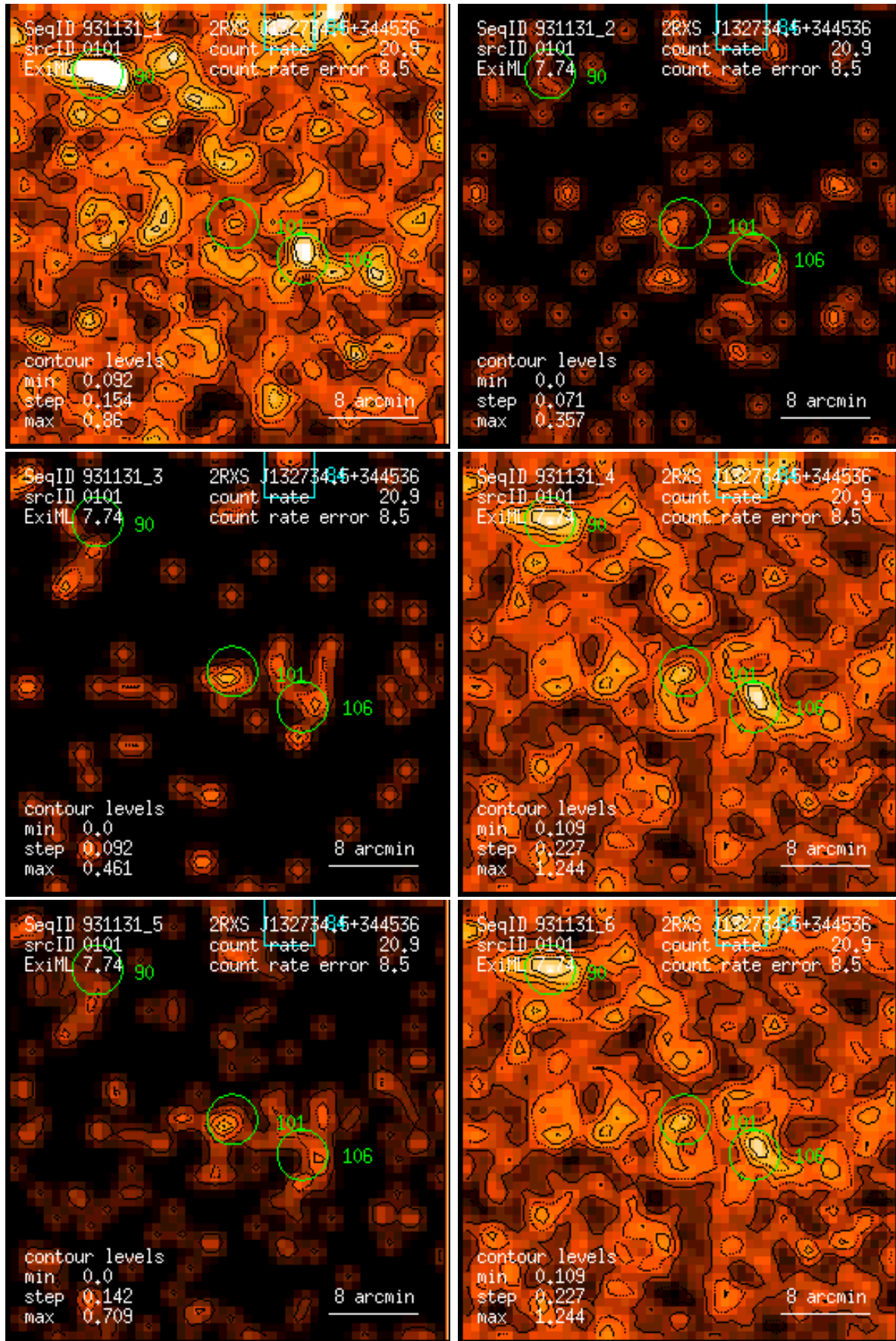
Figure 101: RASS 931131: detection 0101: band rate images, Gaussian filter: (1) PSPC channels 11 – 41, (2) 52 – 90, (3) 91 – 201, (4) 11 – 235, (5) 52 – 201, (6) 11 – 201. Broad band rates in counts/ks. Band rate contour levels in counts/ks/arcmin 2 .
