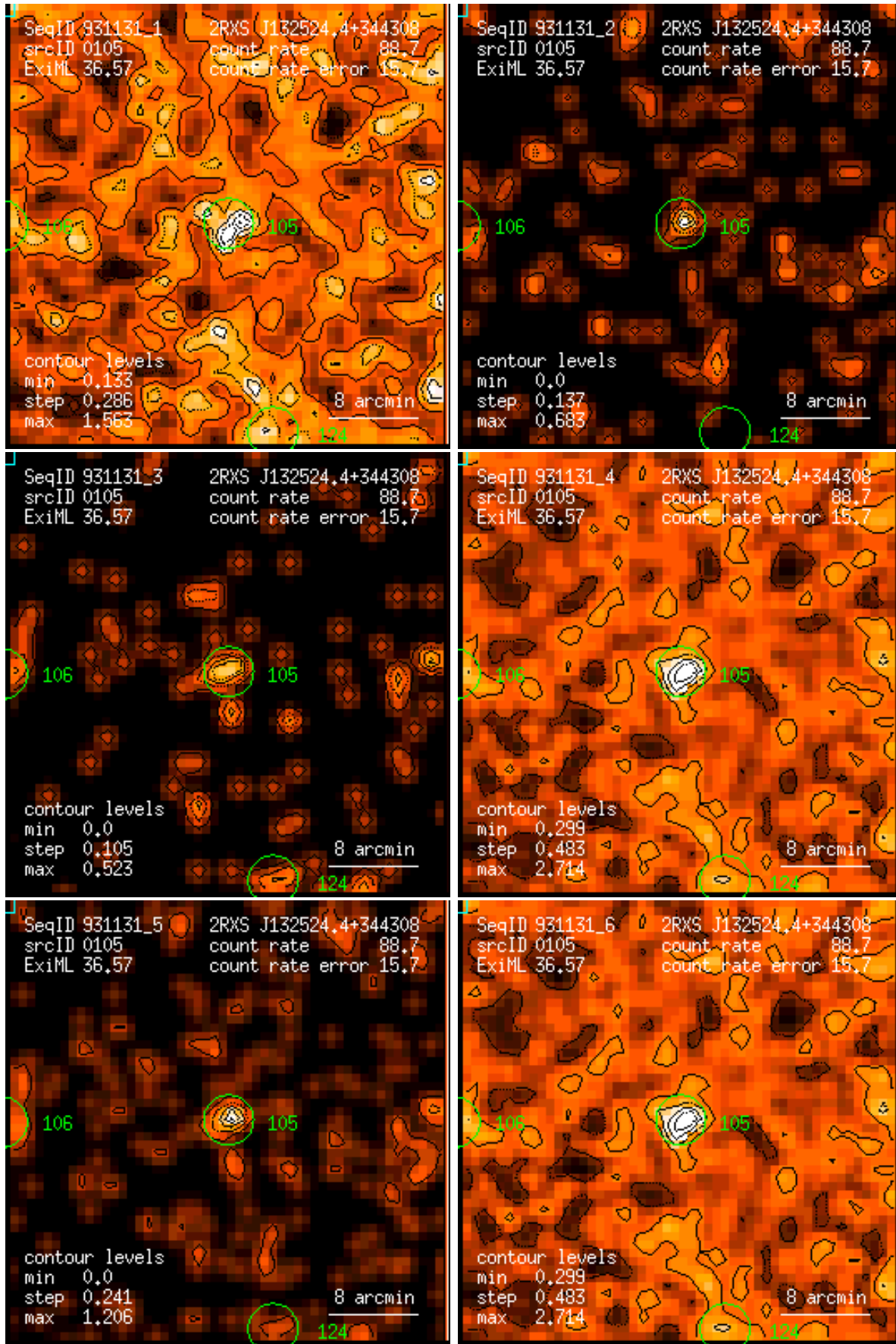
Figure 105: RASS 931131: detection 0105: band rate images, Gaussian filter: (1) PSPC channels 11 – 41, (2) 52 – 90, (3) 91 – 201, (4) 11 – 235, (5) 52 – 201, (6) 11 – 201. Broad band rates in counts/ks. Band rate contour levels in counts/ks/arcmin 2 .
