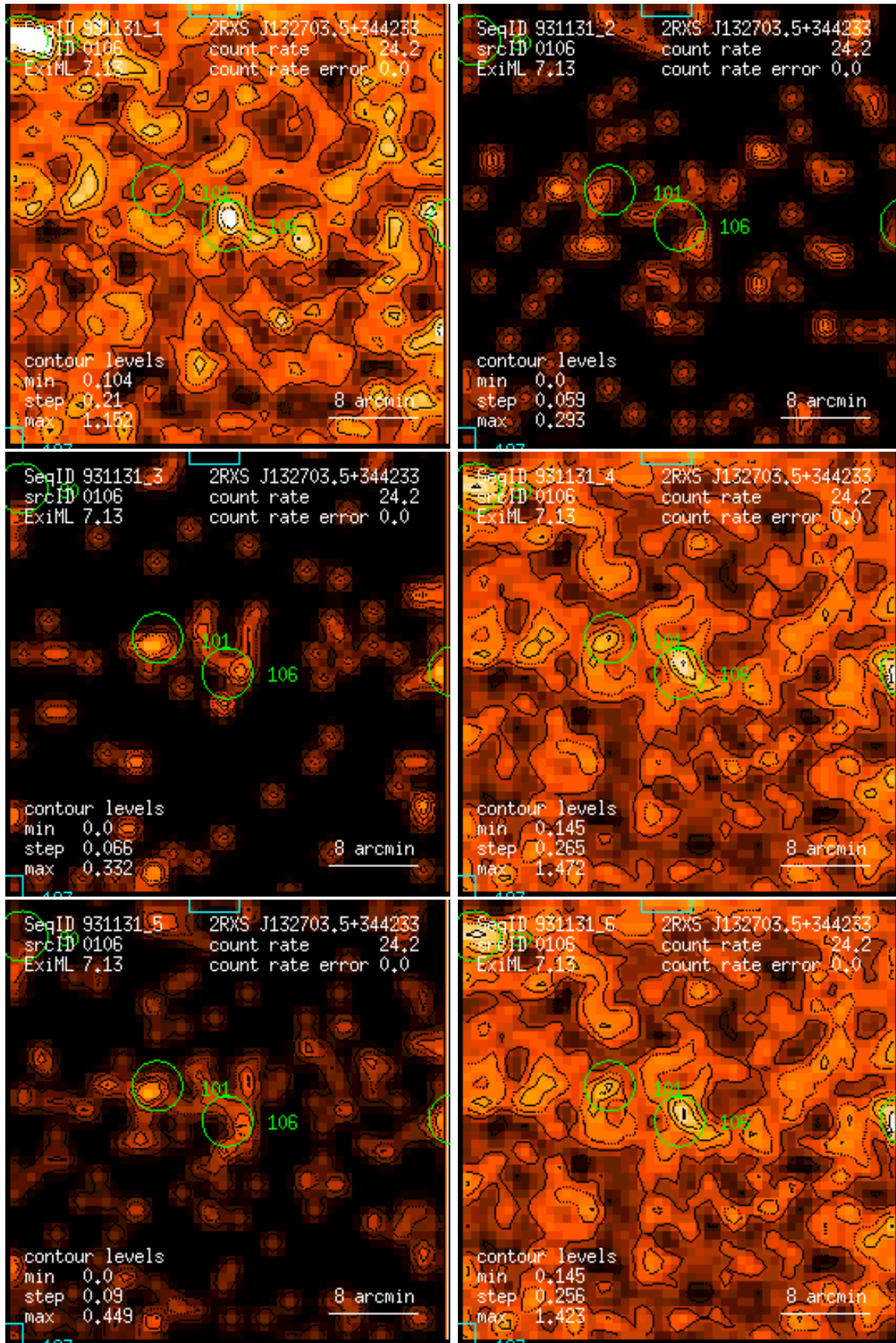
Figure 106: RASS 931131: detection 0106: band rate images, Gaussian filter: (1) PSPC channels 11 – 41, (2) 52 – 90, (3) 91 – 201, (4) 11 – 235, (5) 52 – 201, (6) 11 – 201. Broad band rates in counts/ks. Band rate contour levels in counts/ks/arcmin 2 .
