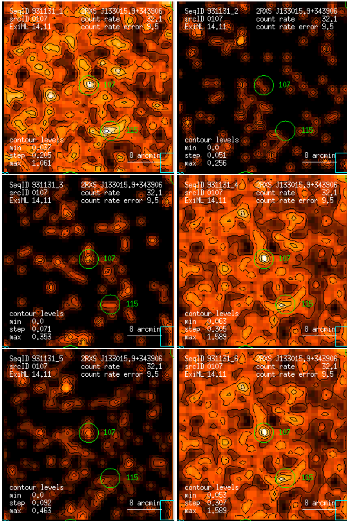
Figure 107: RASS 931131: detection 0107: band rate images, Gaussian filter: (1) PSPC channels 11 – 41, (2) 52 – 90, (3) 91 – 201, (4) 11 – 235, (5) 52 – 201, (6) 11 – 201. Broad band rates in counts/ks. Band rate contour levels in counts/ks/arcmin 2 .
