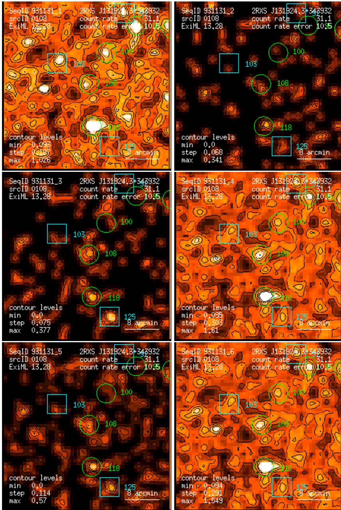
Figure 108: RASS 931131: detection 0108: band rate images, Gaussian filter: (1) PSPC channels 11 – 41, (2) 52 – 90, (3) 91 – 201, (4) 11 – 235, (5) 52 – 201, (6) 11 – 201. Broad band rates in counts/ks. Band rate contour levels in counts/ks/arcmin 2 .
