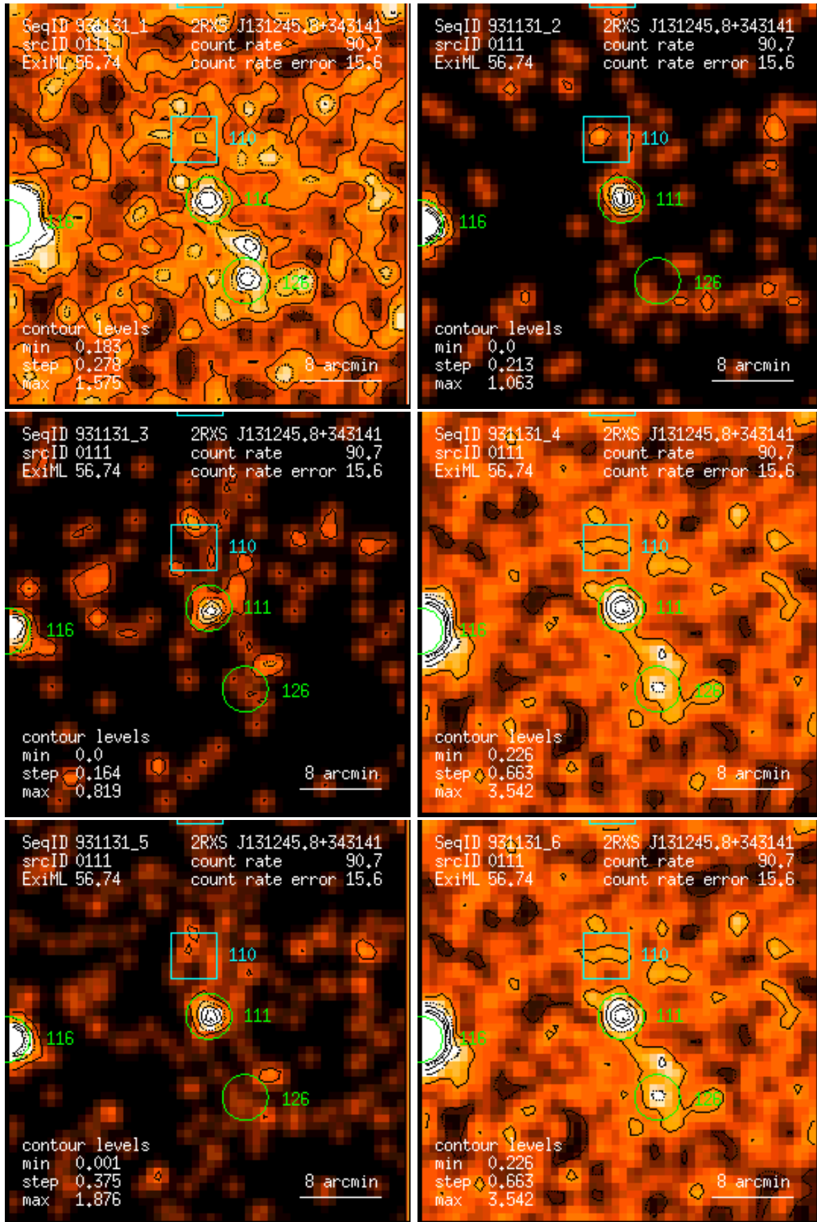
Figure 111: RASS 931131: detection 0111: band rate images, Gaussian filter: (1) PSPC channels 11 – 41, (2) 52 – 90, (3) 91 – 201, (4) 11 – 235, (5) 52 – 201, (6) 11 – 201. Broad band rates in counts/ks. Band rate contour levels in counts/ks/arcmin 2 .
