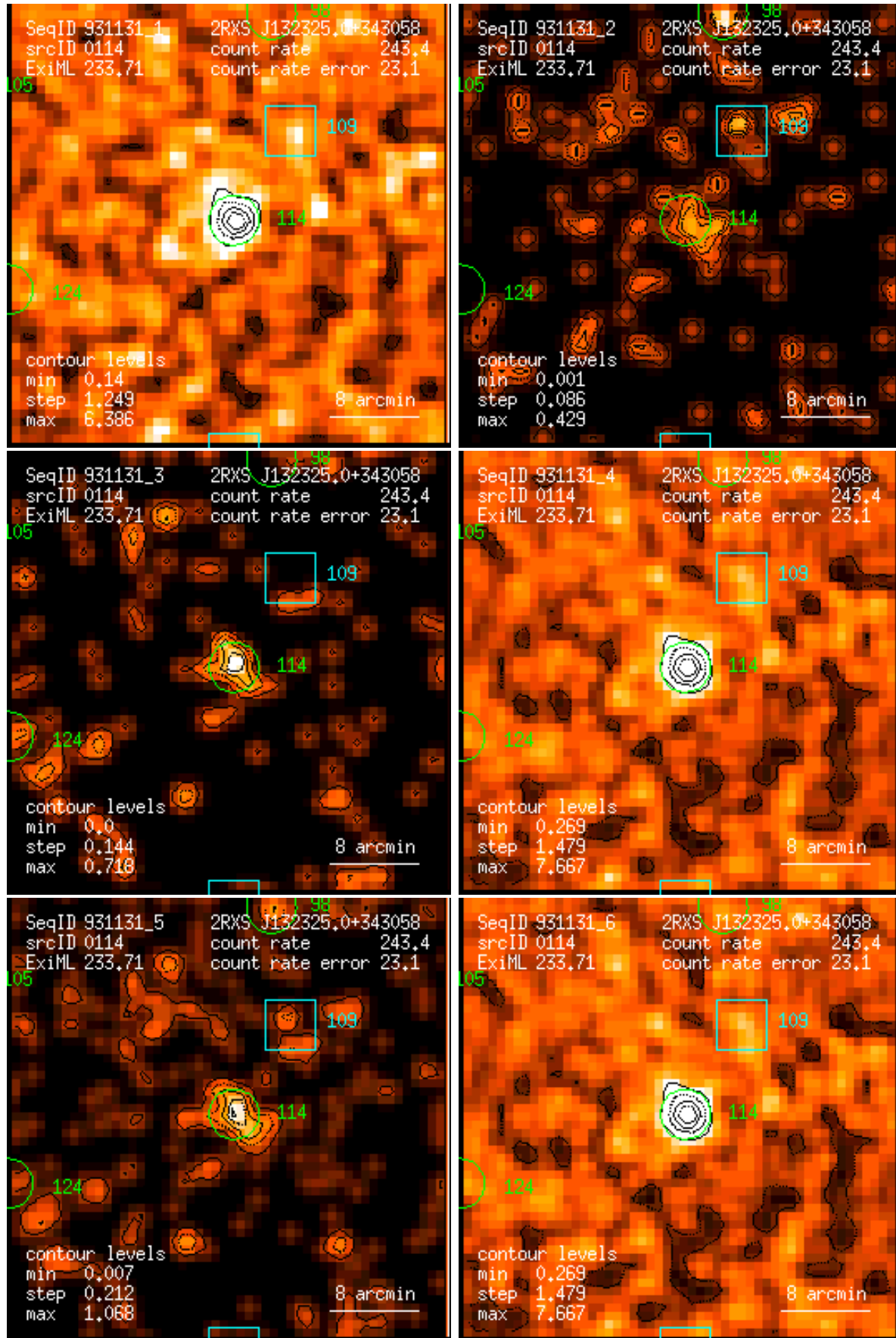
Figure 114: RASS 931131: detection 0114: band rate images, Gaussian filter: (1) PSPC channels 11 – 41, (2) 52 – 90, (3) 91 – 201, (4) 11 – 235, (5) 52 – 201, (6) 11 – 201. Broad band rates in counts/ks. Band rate contour levels in counts/ks/arcmin 2 .
