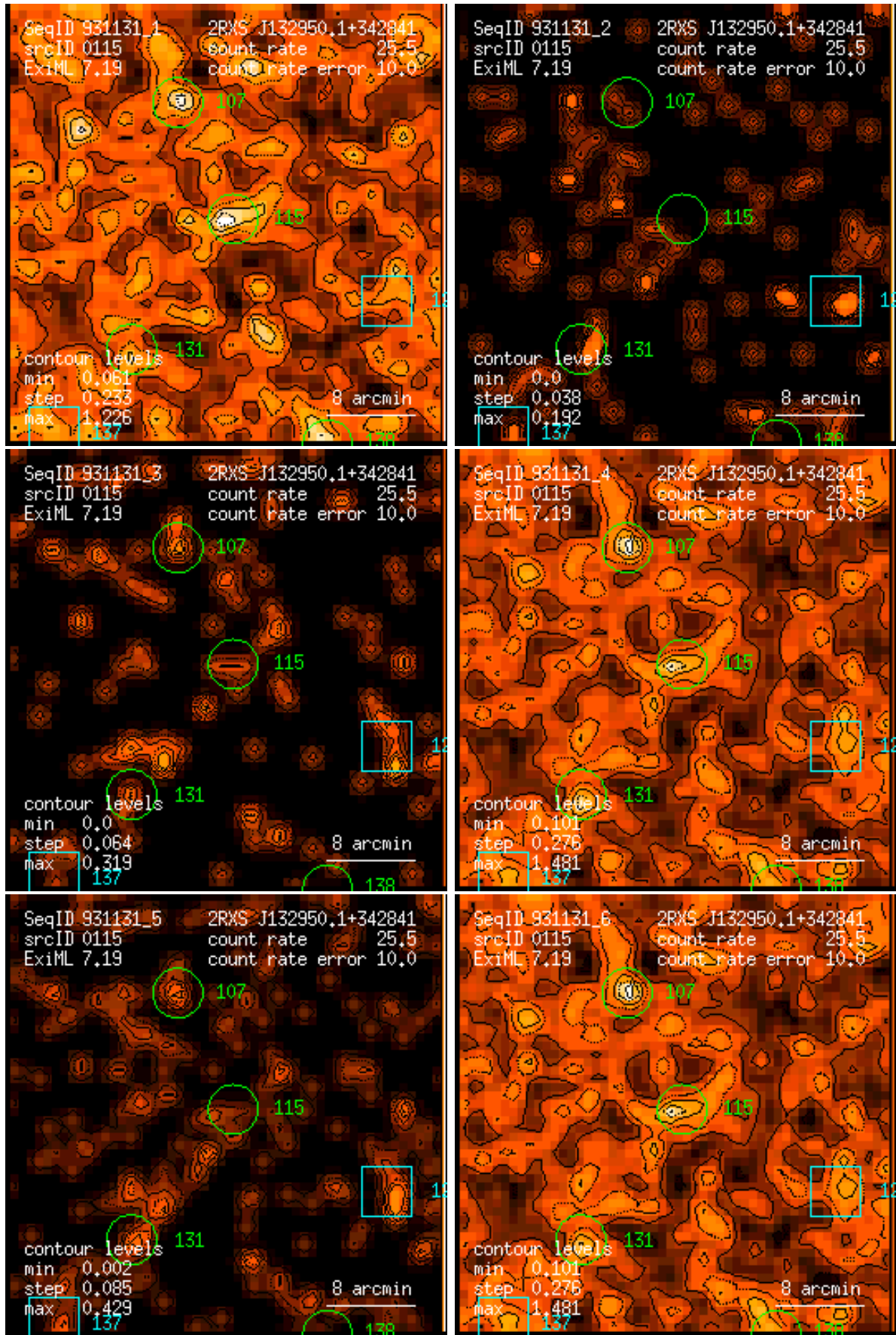
Figure 115: RASS 931131: detection 0115: band rate images, Gaussian filter: (1) PSPC channels 11 – 41, (2) 52 – 90, (3) 91 – 201, (4) 11 – 235, (5) 52 – 201, (6) 11 – 201. Broad band rates in counts/ks. Band rate contour levels in counts/ks/arcmin 2 .
