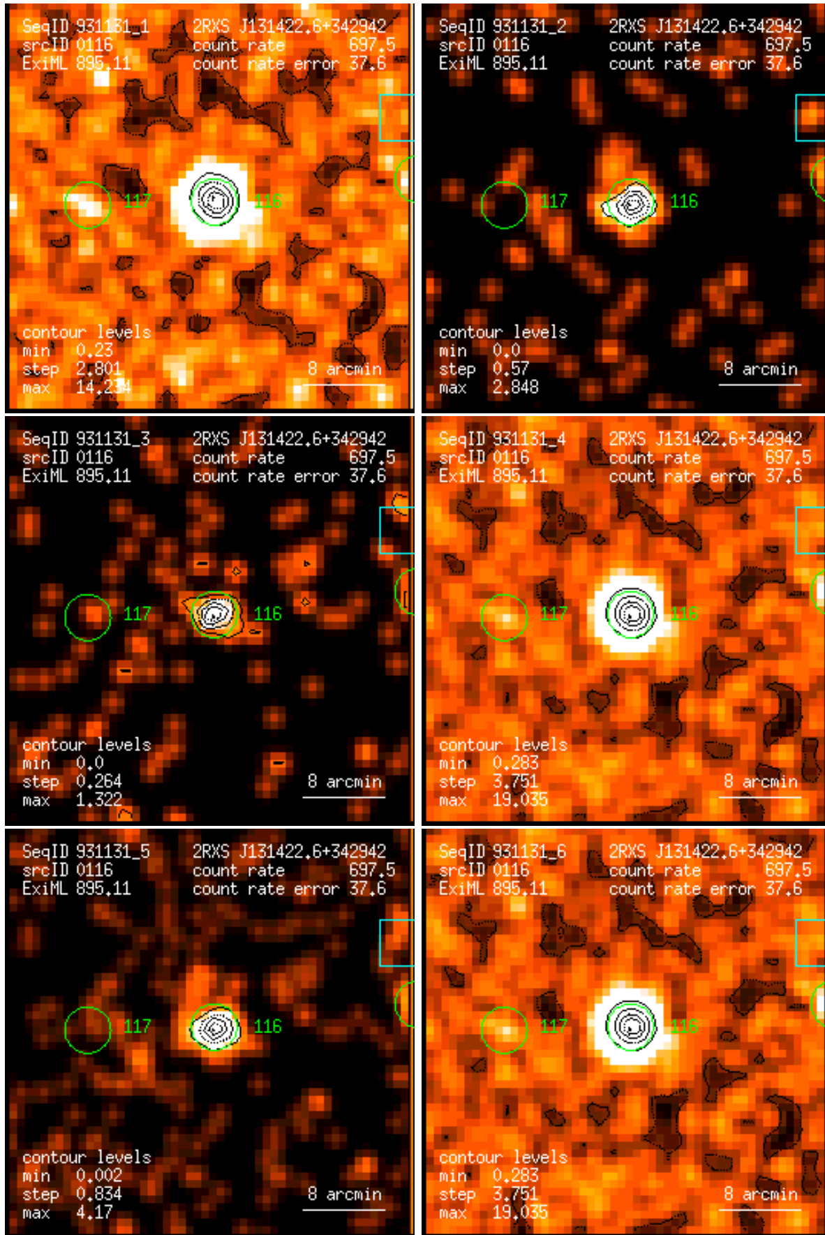
Figure 116: RASS 931131: detection 0116: band rate images, Gaussian filter: (1) PSPC channels 11 – 41, (2) 52 – 90, (3) 91 – 201, (4) 11 – 235, (5) 52 – 201, (6) 11 – 201. Broad band rates in counts/ks. Band rate contour levels in counts/ks/arcmin 2 .
