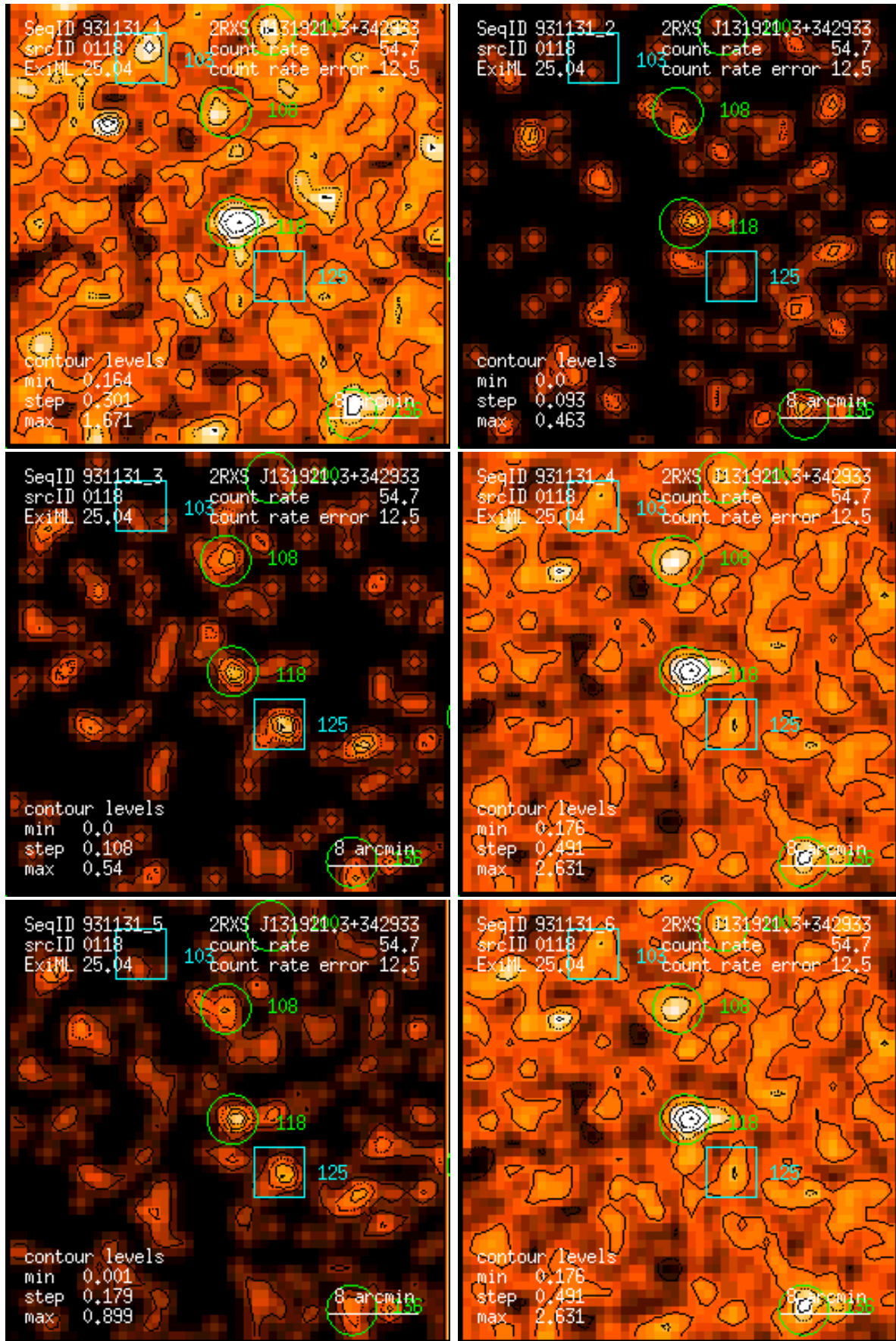
Figure 118: RASS 931131: detection 0118: band rate images, Gaussian filter: (1) PSPC channels 11 – 41, (2) 52 – 90, (3) 91 – 201, (4) 11 – 235, (5) 52 – 201, (6) 11 – 201. Broad band rates in counts/ks. Band rate contour levels in counts/ks/arcmin 2 .
