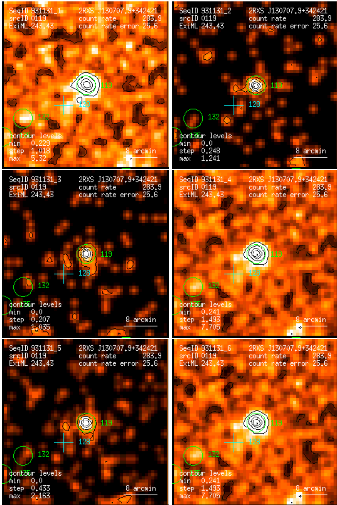
Figure 119: RASS 931131: detection 0119: band rate images, Gaussian filter: (1) PSPC channels 11 – 41, (2) 52 – 90, (3) 91 – 201, (4) 11 – 235, (5) 52 – 201, (6) 11 – 201. Broad band rates in counts/ks. Band rate contour levels in counts/ks/arcmin 2 .
