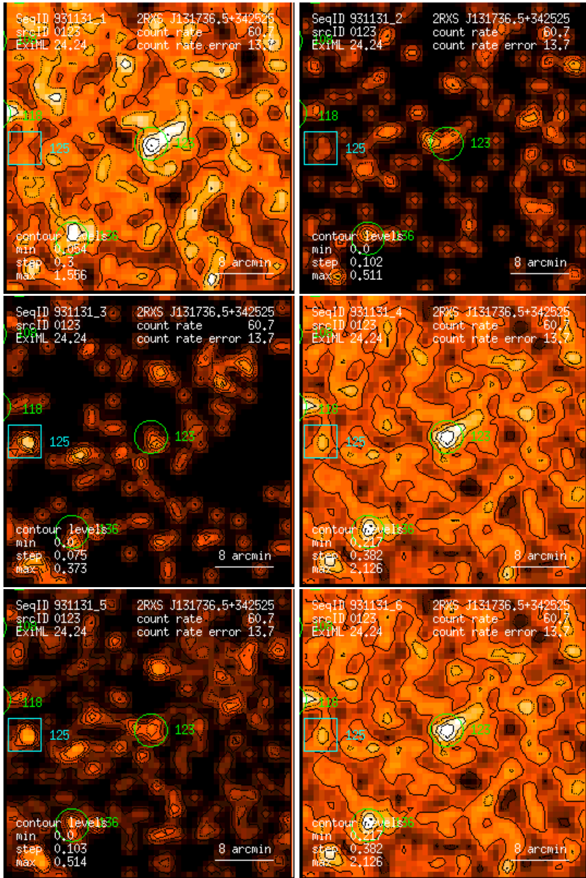
Figure 123: RASS 931131: detection 0123: band rate images, Gaussian filter: (1) PSPC channels 11 – 41, (2) 52 – 90, (3) 91 – 201, (4) 11 – 235, (5) 52 – 201, (6) 11 – 201. Broad band rates in counts/ks. Band rate contour levels in counts/ks/arcmin 2 .
