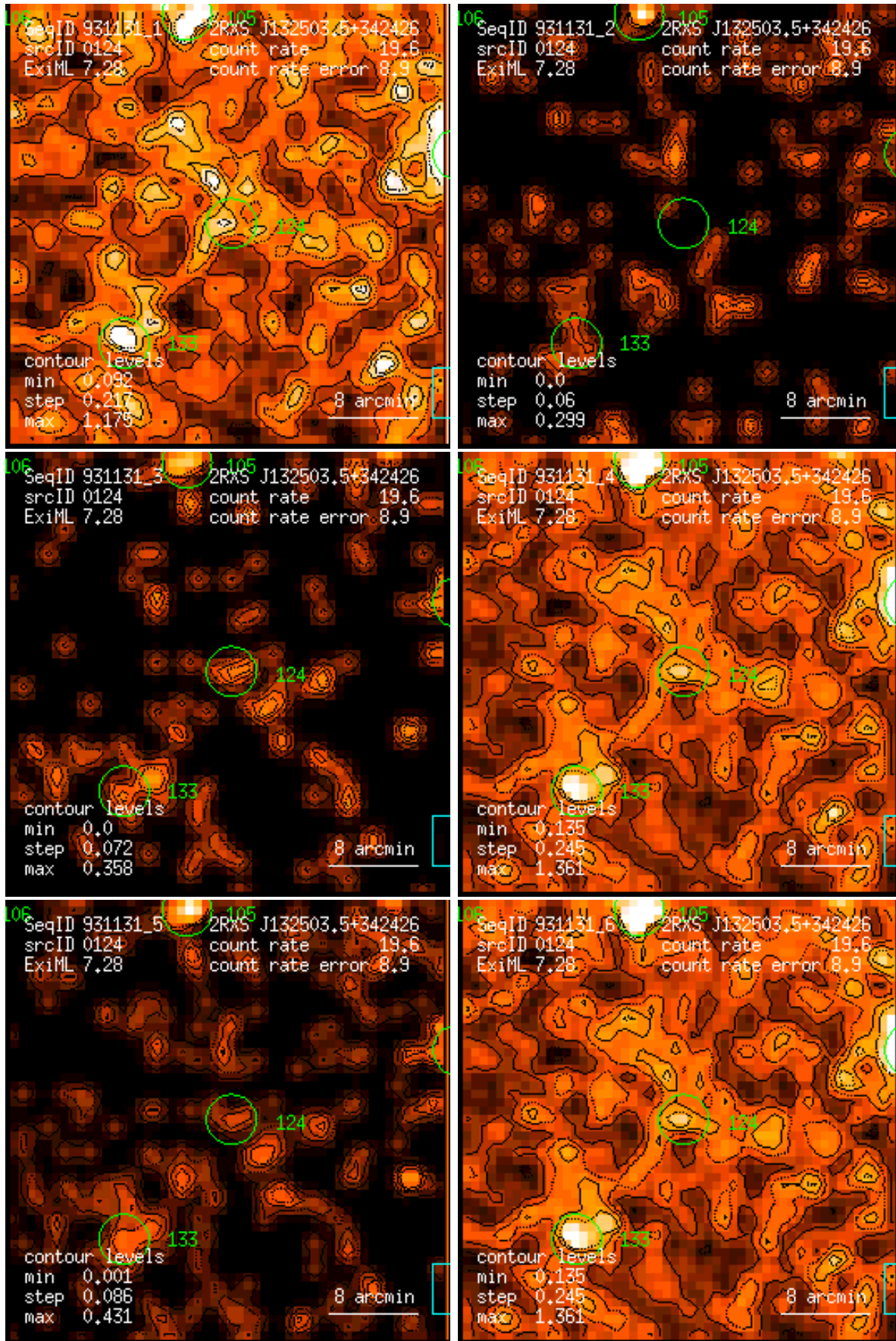
Figure 124: RASS 931131: detection 0124: band rate images, Gaussian filter: (1) PSPC channels 11 – 41, (2) 52 – 90, (3) 91 – 201, (4) 11 – 235, (5) 52 – 201, (6) 11 – 201. Broad band rates in counts/ks. Band rate contour levels in counts/ks/arcmin 2 .
