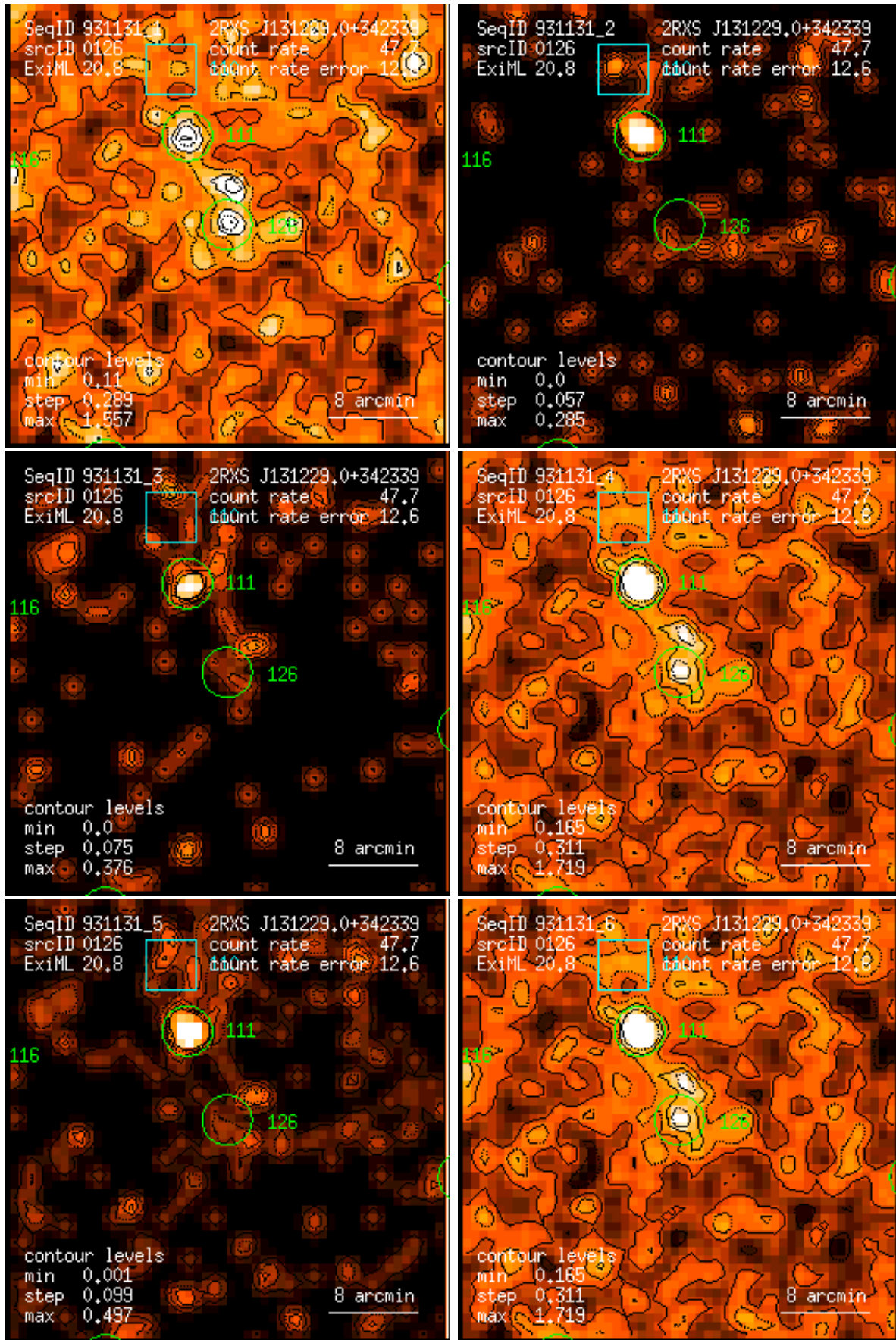
Figure 126: RASS 931131: detection 0126: band rate images, Gaussian filter: (1) PSPC channels 11 – 41, (2) 52 – 90, (3) 91 – 201, (4) 11 – 235, (5) 52 – 201, (6) 11 – 201. Broad band rates in counts/ks. Band rate contour levels in counts/ks/arcmin 2 .
