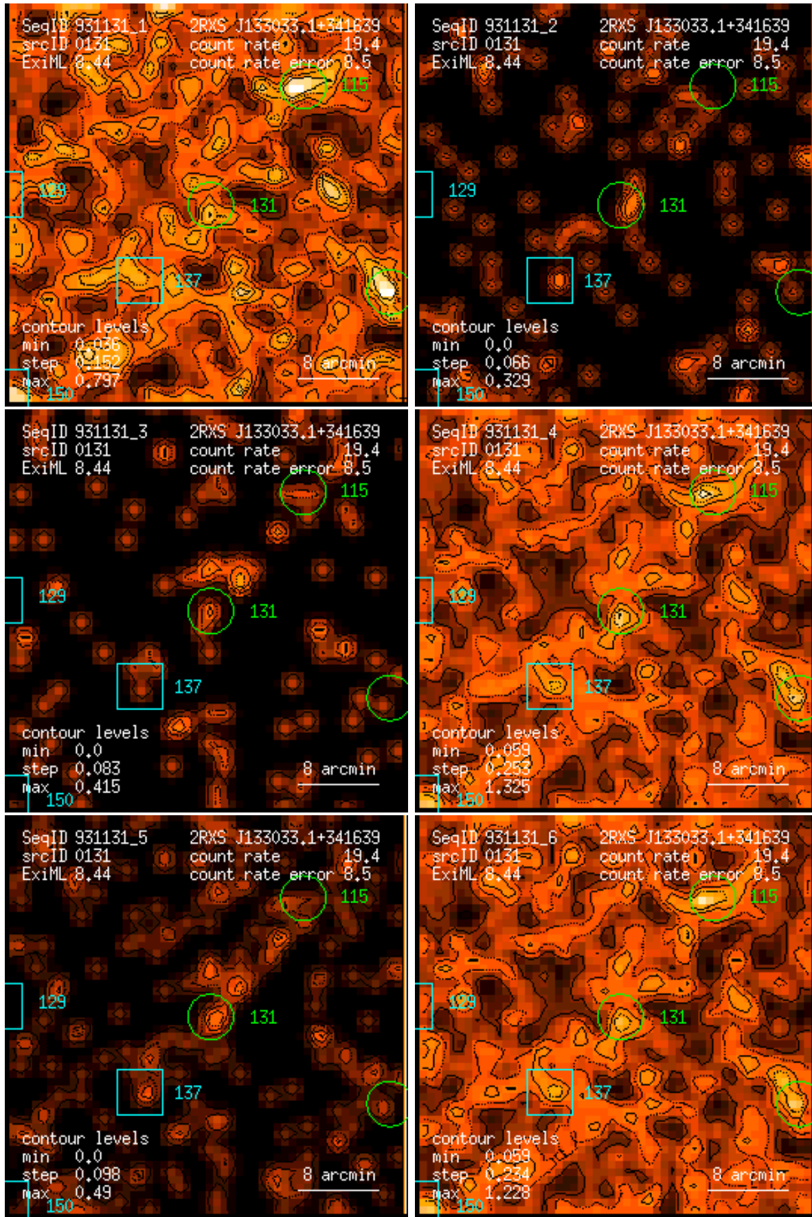
Figure 131: RASS 931131: detection 0131: band rate images, Gaussian filter: (1) PSPC channels 11 – 41, (2) 52 – 90, (3) 91 – 201, (4) 11 – 235, (5) 52 – 201, (6) 11 – 201. Broad band rates in counts/ks. Band rate contour levels in counts/ks/arcmin 2 .
