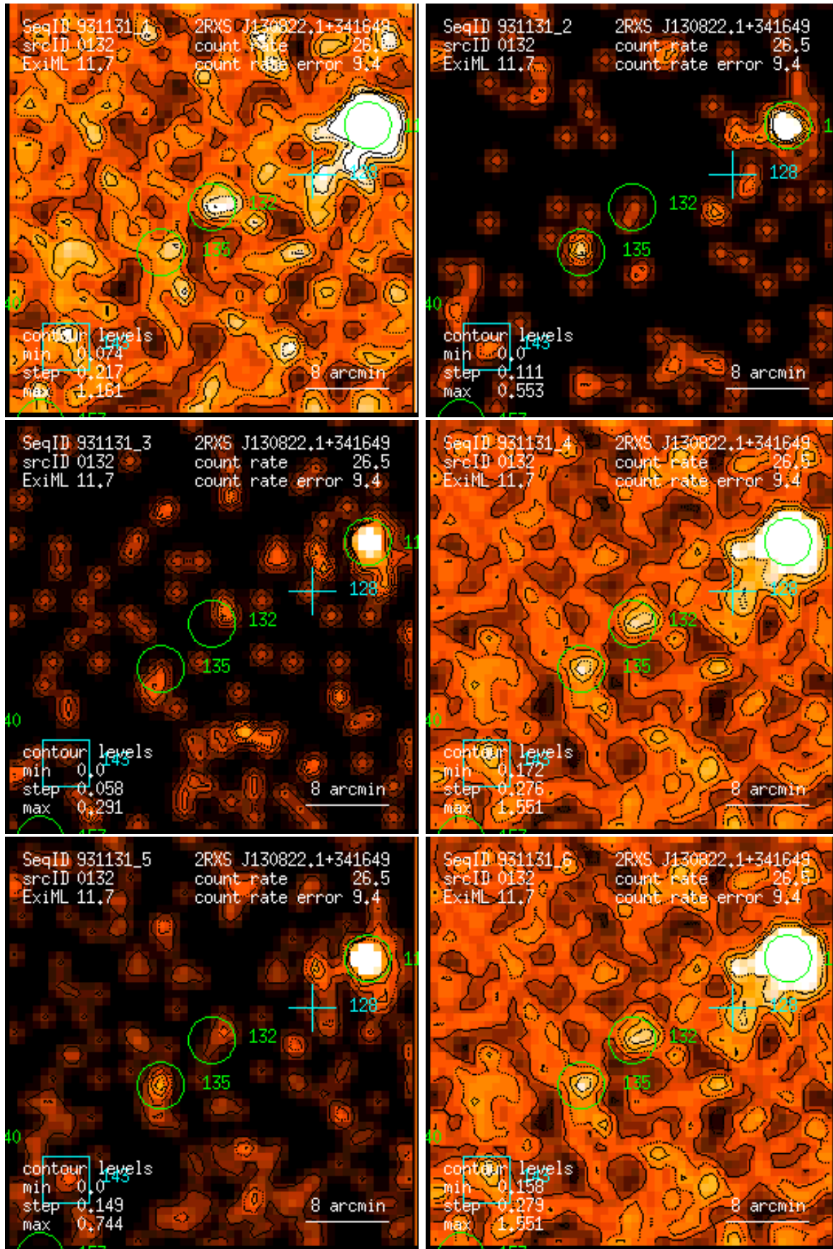
Figure 132: RASS 931131: detection 0132: band rate images, Gaussian filter: (1) PSPC channels 11 – 41, (2) 52 – 90, (3) 91 – 201, (4) 11 – 235, (5) 52 – 201, (6) 11 – 201. Broad band rates in counts/ks. Band rate contour levels in counts/ks/arcmin 2 .
