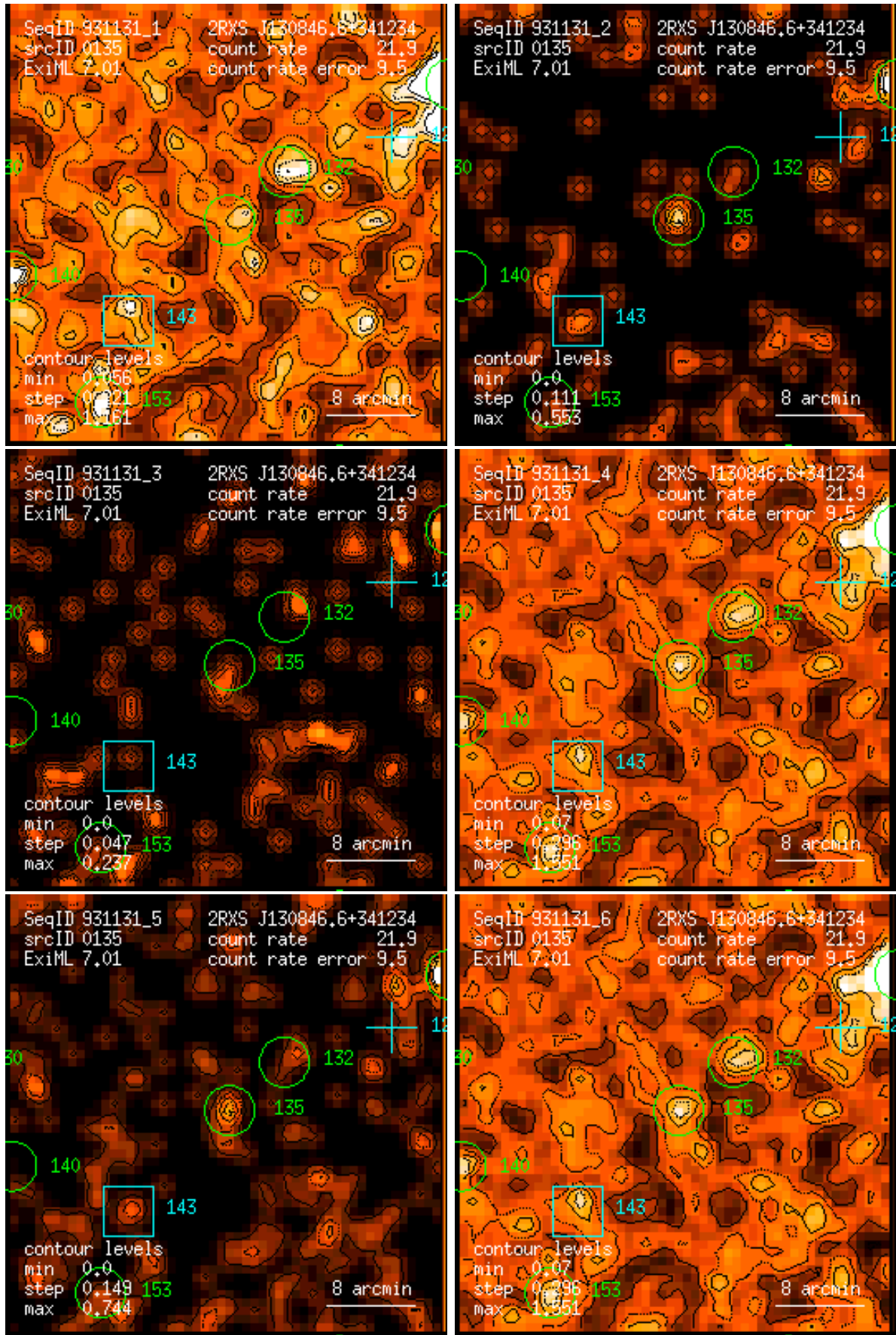
Figure 135: RASS 931131: detection 0135: band rate images, Gaussian filter: (1) PSPC channels 11 – 41, (2) 52 – 90, (3) 91 – 201, (4) 11 – 235, (5) 52 – 201, (6) 11 – 201. Broad band rates in counts/ks. Band rate contour levels in counts/ks/arcmin 2 .
