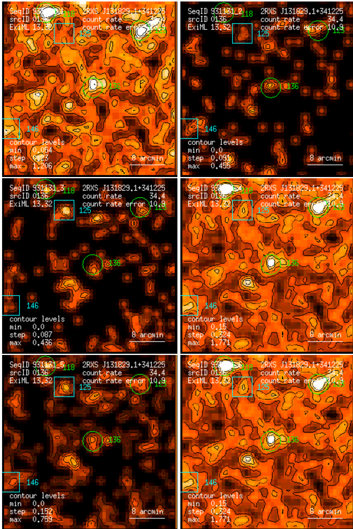
Figure 136: RASS 931131: detection 0136: band rate images, Gaussian filter: (1) PSPC channels 11 – 41, (2) 52 – 90, (3) 91 – 201, (4) 11 – 235, (5) 52 – 201, (6) 11 – 201. Broad band rates in counts/ks. Band rate contour levels in counts/ks/arcmin 2 .
