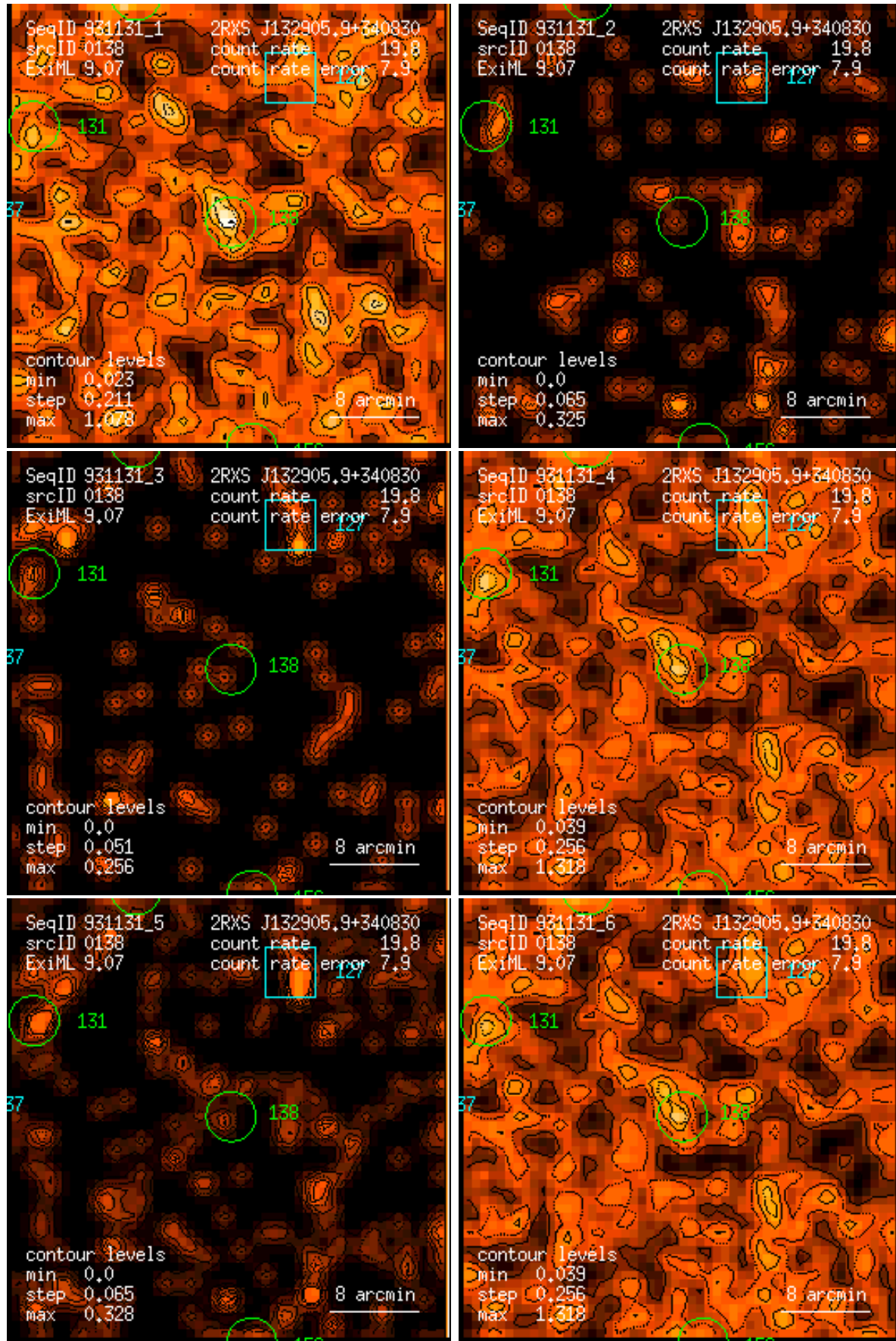
Figure 138: RASS 931131: detection 0138: band rate images, Gaussian filter: (1) PSPC channels 11 – 41, (2) 52 – 90, (3) 91 – 201, (4) 11 – 235, (5) 52 – 201, (6) 11 – 201. Broad band rates in counts/ks. Band rate contour levels in counts/ks/arcmin 2 .
