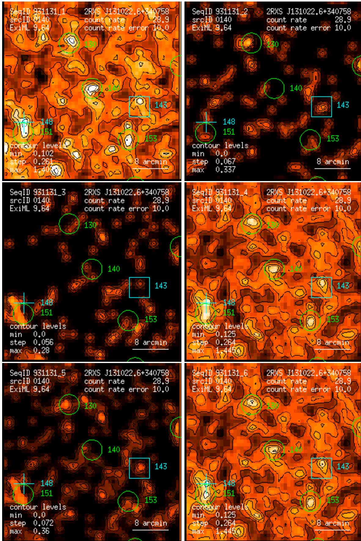
Figure 140: RASS 931131: detection 0140: band rate images, Gaussian filter: (1) PSPC channels 11 – 41, (2) 52 – 90, (3) 91 – 201, (4) 11 – 235, (5) 52 – 201, (6) 11 – 201. Broad band rates in counts/ks. Band rate contour levels in counts/ks/arcmin 2 .
