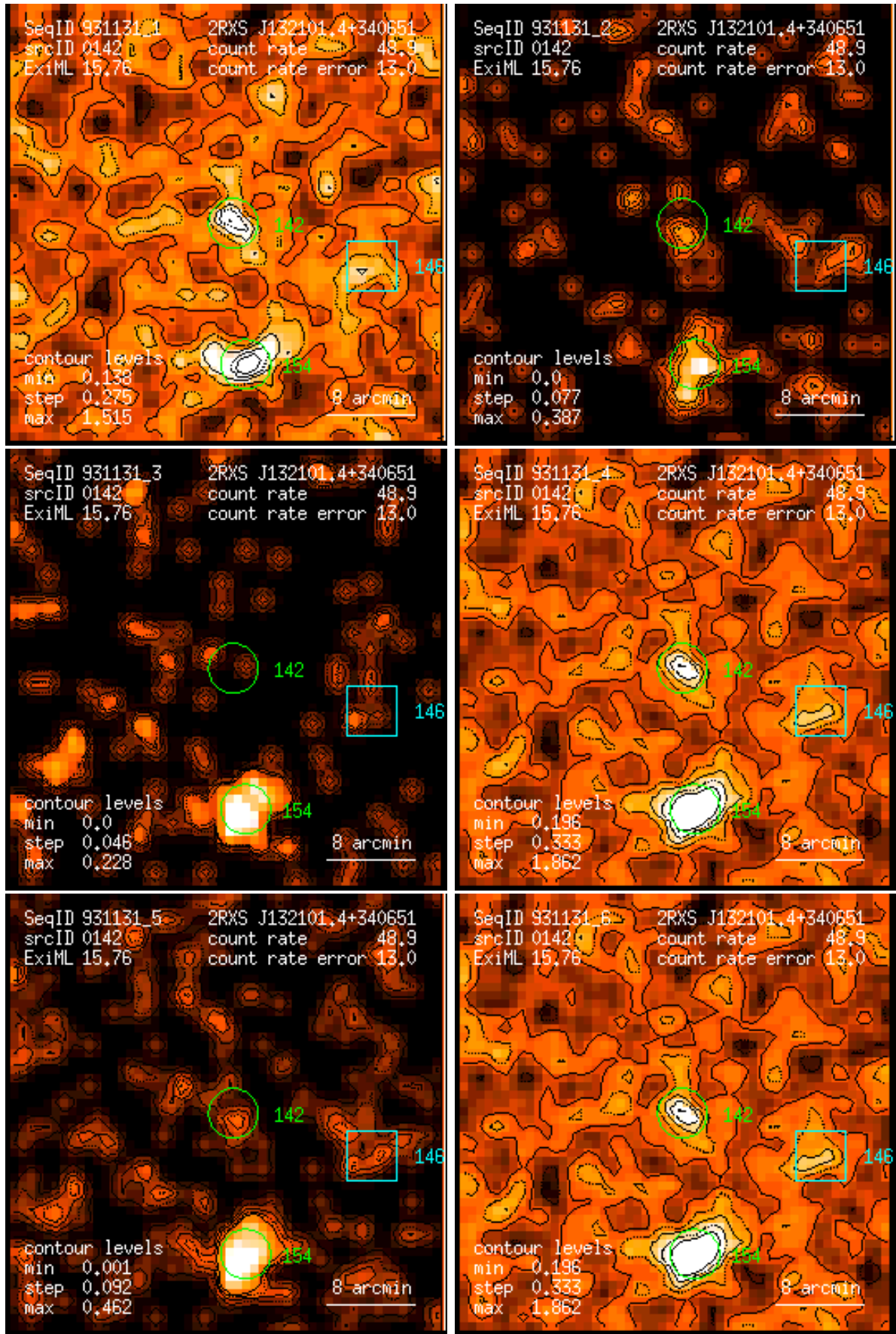
Figure 142: RASS 931131: detection 0142: band rate images, Gaussian filter: (1) PSPC channels 11 – 41, (2) 52 – 90, (3) 91 – 201, (4) 11 – 235, (5) 52 – 201, (6) 11 – 201. Broad band rates in counts/ks. Band rate contour levels in counts/ks/arcmin 2 .
