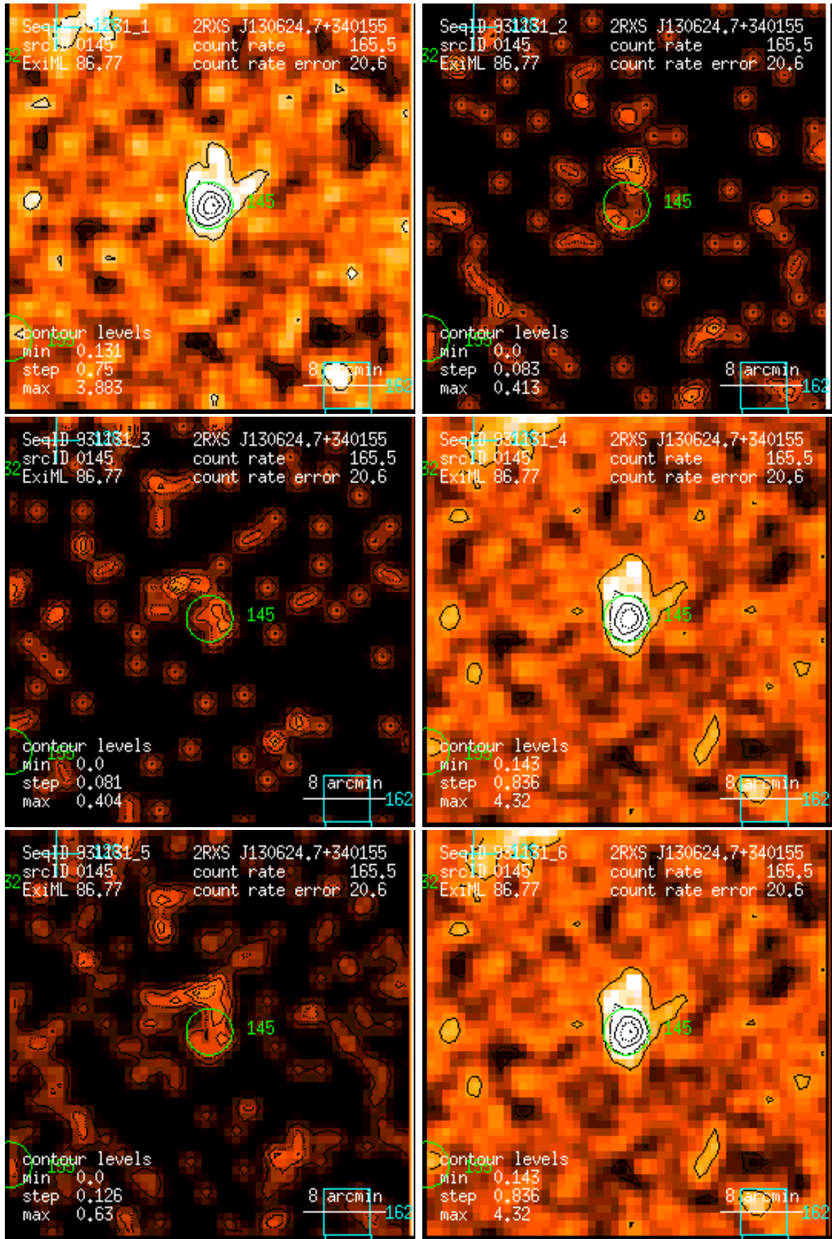
Figure 145: RASS 931131: detection 0145: band rate images, Gaussian filter: (1) PSPC channels 11 – 41, (2) 52 – 90, (3) 91 – 201, (4) 11 – 235, (5) 52 – 201, (6) 11 – 201. Broad band rates in counts/ks. Band rate contour levels in counts/ks/arcmin 2 .
