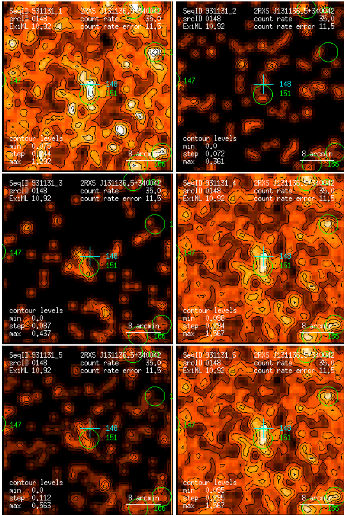
Figure 148: RASS 931131: detection 0148: band rate images, Gaussian filter: (1) PSPC channels 11 – 41, (2) 52 – 90, (3) 91 – 201, (4) 11 – 235, (5) 52 – 201, (6) 11 – 201. Broad band rates in counts/ks. Band rate contour levels in counts/ks/arcmin 2 .
