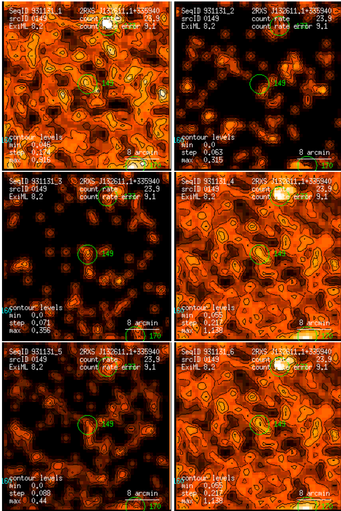
Figure 149: RASS 931131: detection 0149: band rate images, Gaussian filter: (1) PSPC channels 11 – 41, (2) 52 – 90, (3) 91 – 201, (4) 11 – 235, (5) 52 – 201, (6) 11 – 201. Broad band rates in counts/ks. Band rate contour levels in counts/ks/arcmin 2 .
