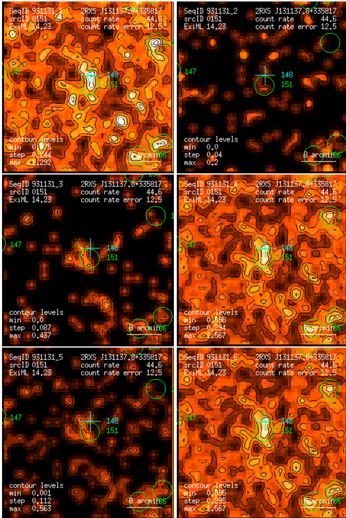
Figure 151: RASS 931131: detection 0151: band rate images, Gaussian filter: (1) PSPC channels 11 – 41, (2) 52 – 90, (3) 91 – 201, (4) 11 – 235, (5) 52 – 201, (6) 11 – 201. Broad band rates in counts/ks. Band rate contour levels in counts/ks/arcmin 2 .
