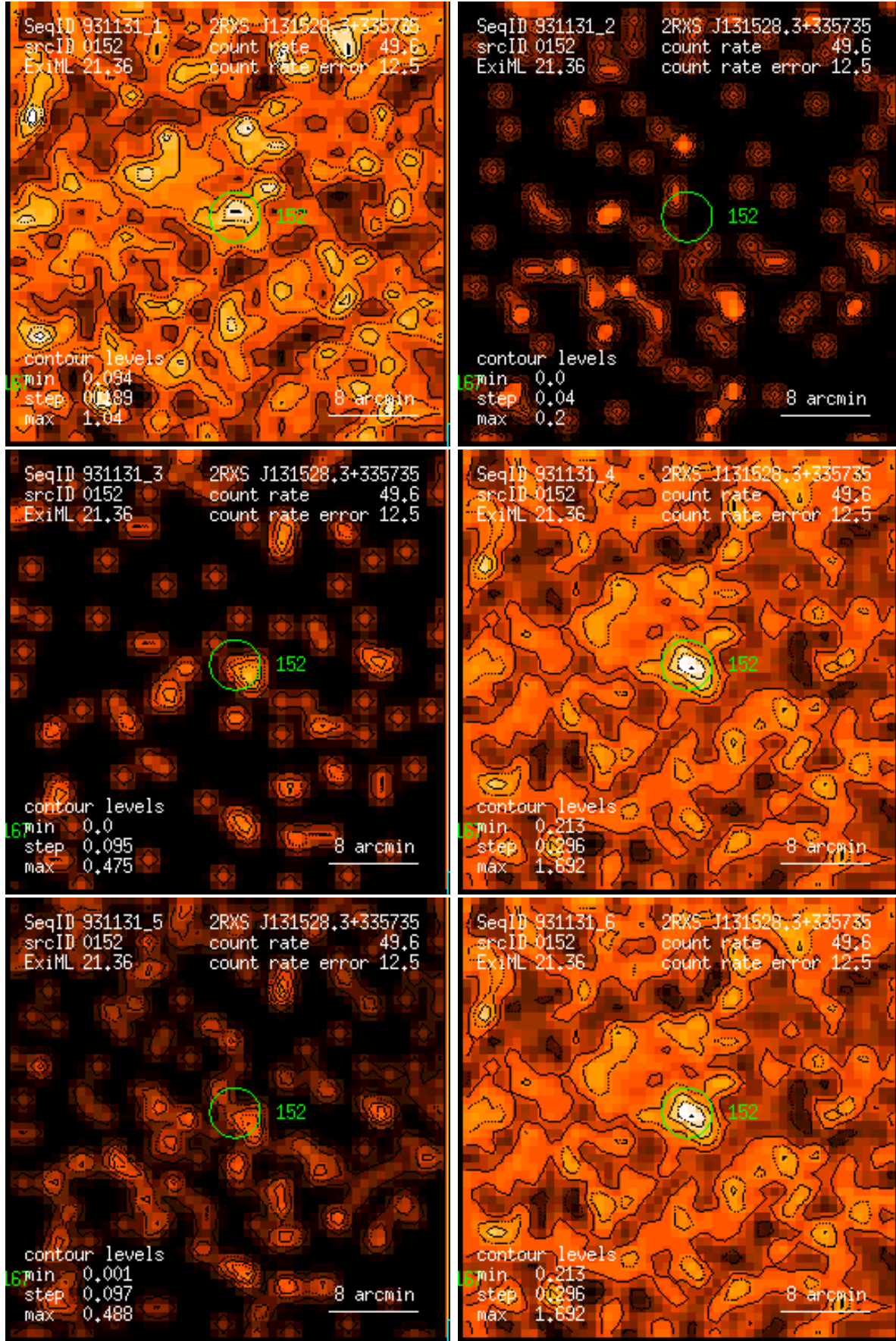
Figure 152: RASS 931131: detection 0152: band rate images, Gaussian filter: (1) PSPC channels 11 – 41, (2) 52 – 90, (3) 91 – 201, (4) 11 – 235, (5) 52 – 201, (6) 11 – 201. Broad band rates in counts/ks. Band rate contour levels in counts/ks/arcmin 2 .
