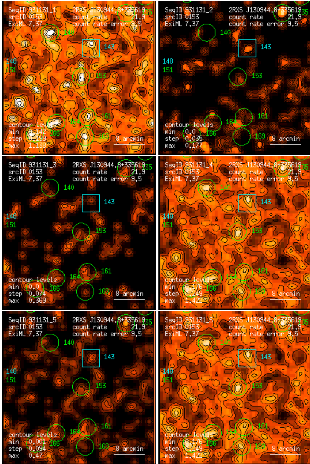
Figure 153: RASS 931131: detection 0153: band rate images, Gaussian filter: (1) PSPC channels 11 – 41, (2) 52 – 90, (3) 91 – 201, (4) 11 – 235, (5) 52 – 201, (6) 11 – 201. Broad band rates in counts/ks. Band rate contour levels in counts/ks/arcmin 2 .
