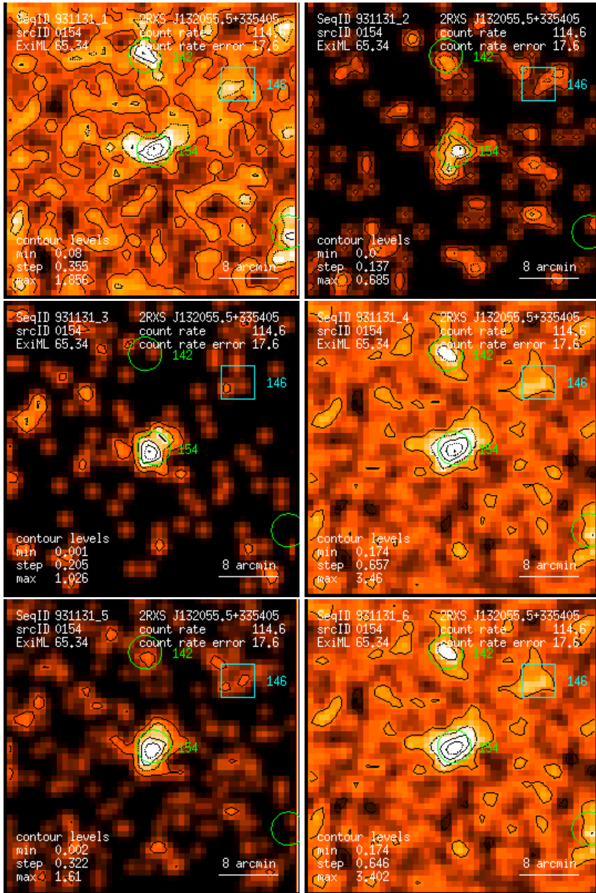
Figure 154: RASS 931131: detection 0154: band rate images, Gaussian filter: (1) PSPC channels 11 – 41, (2) 52 – 90, (3) 91 – 201, (4) 11 – 235, (5) 52 – 201, (6) 11 – 201. Broad band rates in counts/ks. Band rate contour levels in counts/ks/arcmin 2 .
