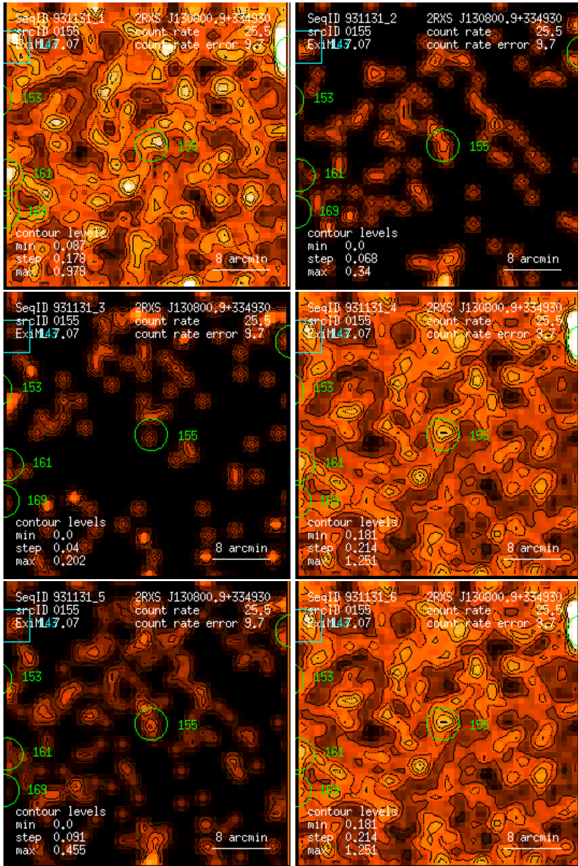
Figure 155: RASS 931131: detection 0155: band rate images, Gaussian filter: (1) PSPC channels 11 – 41, (2) 52 – 90, (3) 91 – 201, (4) 11 – 235, (5) 52 – 201, (6) 11 – 201. Broad band rates in counts/ks. Band rate contour levels in counts/ks/arcmin 2 .
