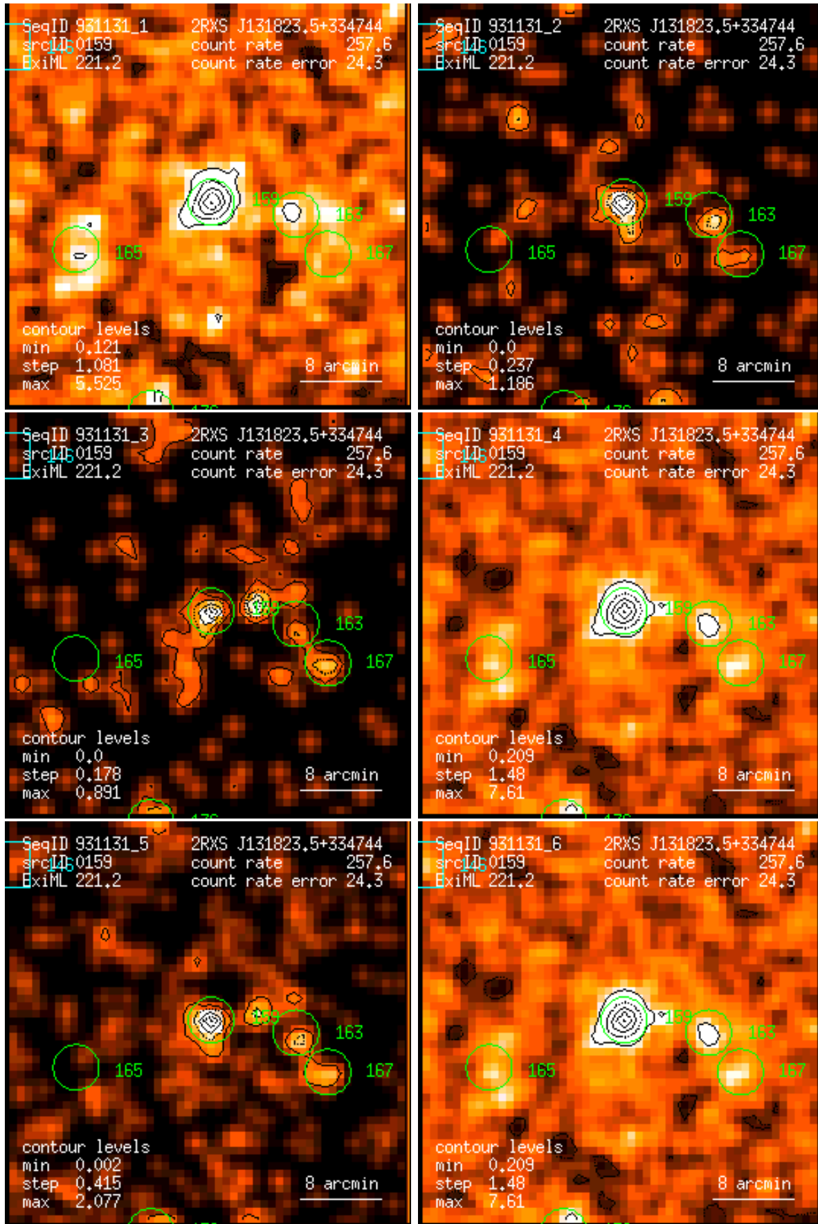
Figure 159: RASS 931131: detection 0159: band rate images, Gaussian filter: (1) PSPC channels 11 – 41, (2) 52 – 90, (3) 91 – 201, (4) 11 – 235, (5) 52 – 201, (6) 11 – 201. Broad band rates in counts/ks. Band rate contour levels in counts/ks/arcmin 2 .
