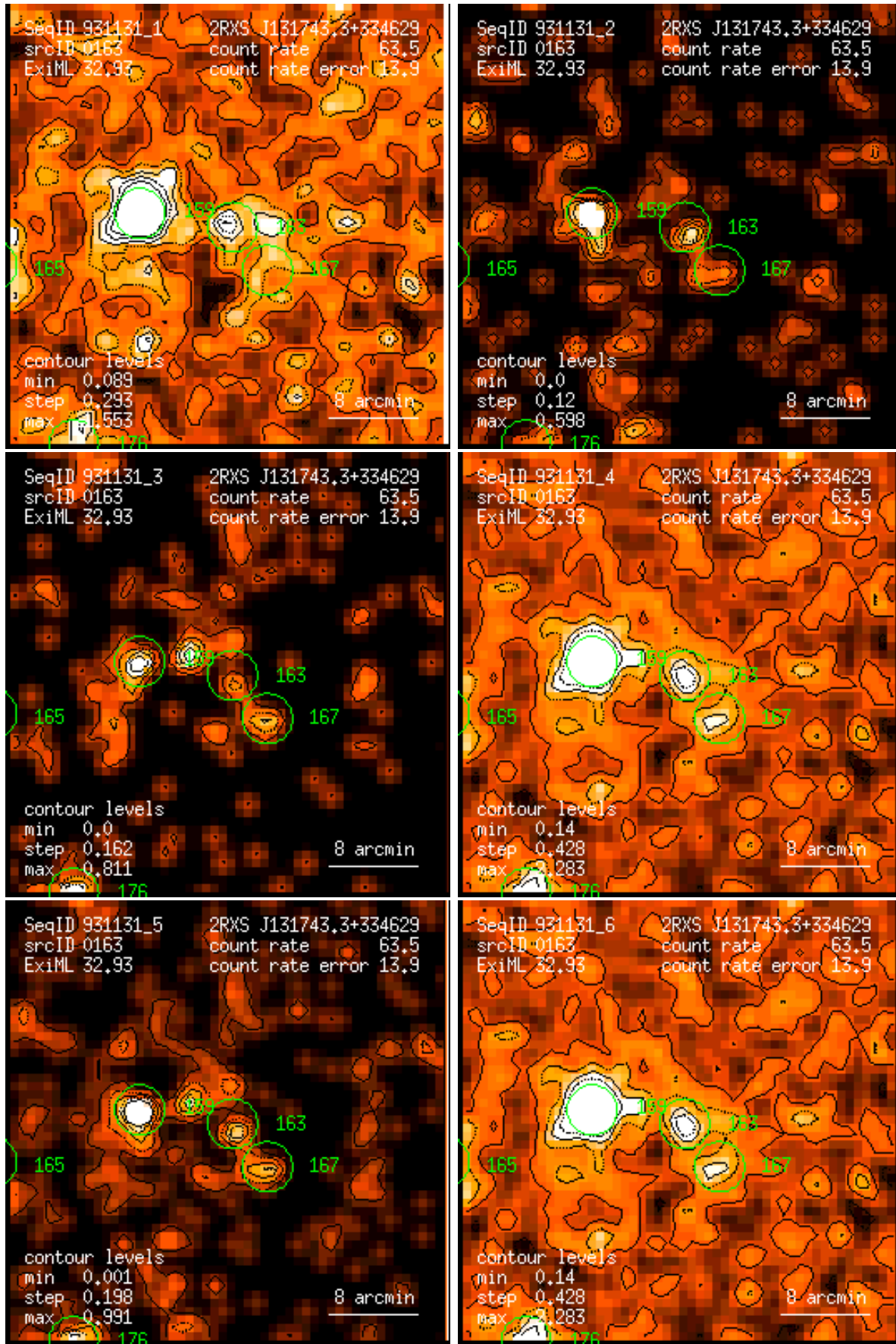
Figure 163: RASS 931131: detection 0163: band rate images, Gaussian filter: (1) PSPC channels 11 – 41, (2) 52 – 90, (3) 91 – 201, (4) 11 – 235, (5) 52 – 201, (6) 11 – 201. Broad band rates in counts/ks. Band rate contour levels in counts/ks/arcmin 2 .
