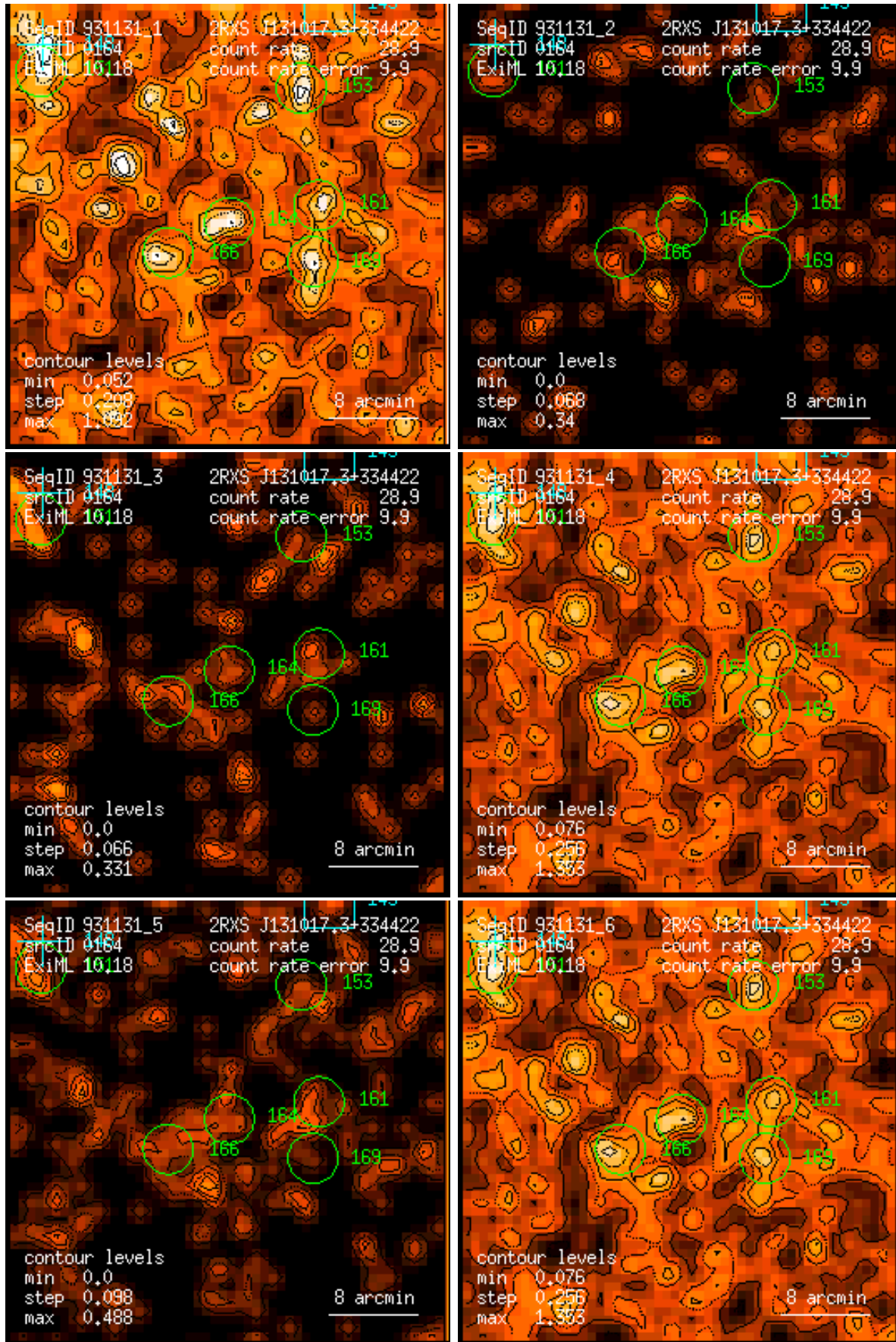
Figure 164: RASS 931131: detection 0164: band rate images, Gaussian filter: (1) PSPC channels 11 – 41, (2) 52 – 90, (3) 91 – 201, (4) 11 – 235, (5) 52 – 201, (6) 11 – 201. Broad band rates in counts/ks. Band rate contour levels in counts/ks/arcmin 2 .
