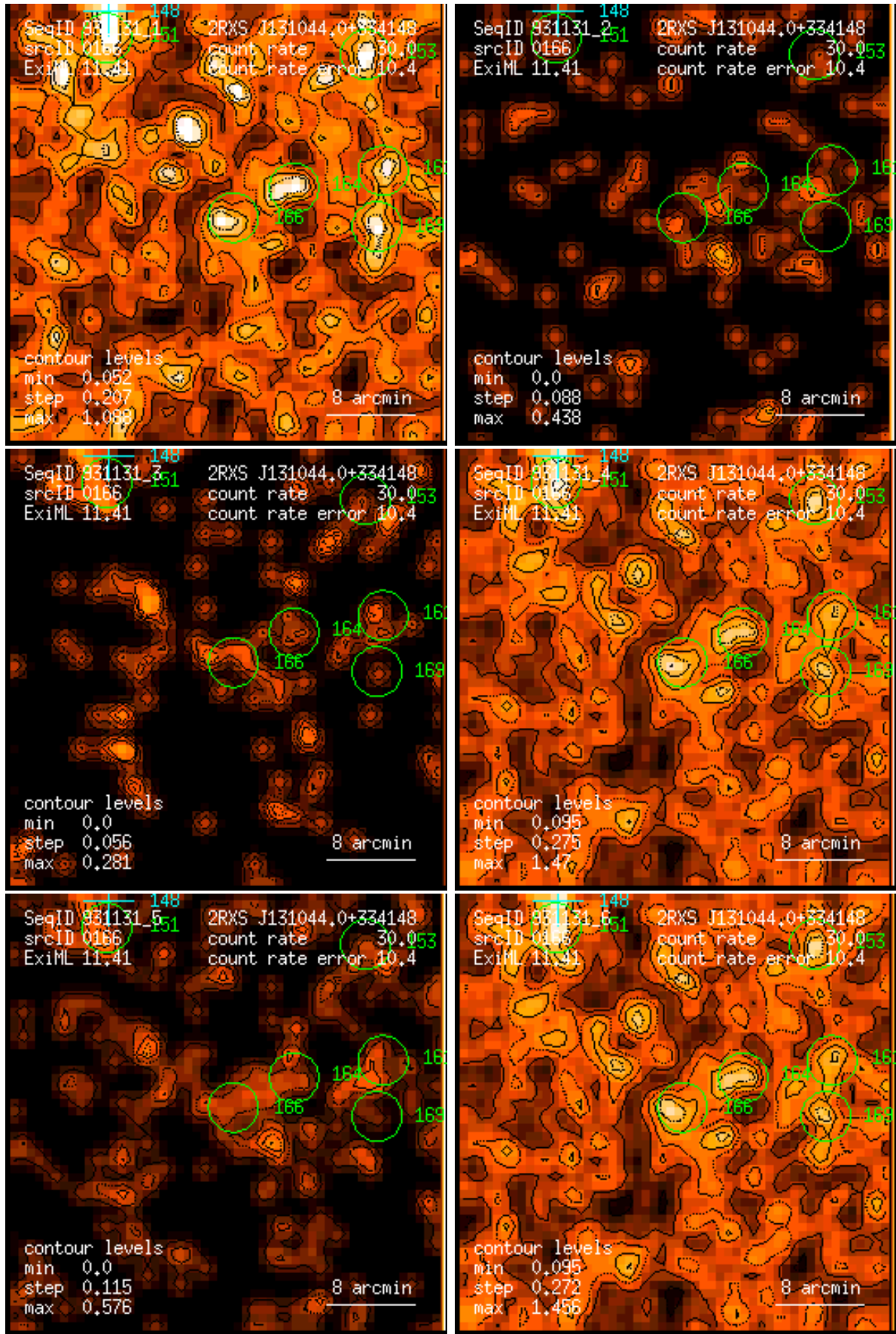
Figure 166: RASS 931131: detection 0166: band rate images, Gaussian filter: (1) PSPC channels 11 – 41, (2) 52 – 90, (3) 91 – 201, (4) 11 – 235, (5) 52 – 201, (6) 11 – 201. Broad band rates in counts/ks. Band rate contour levels in counts/ks/arcmin 2 .
