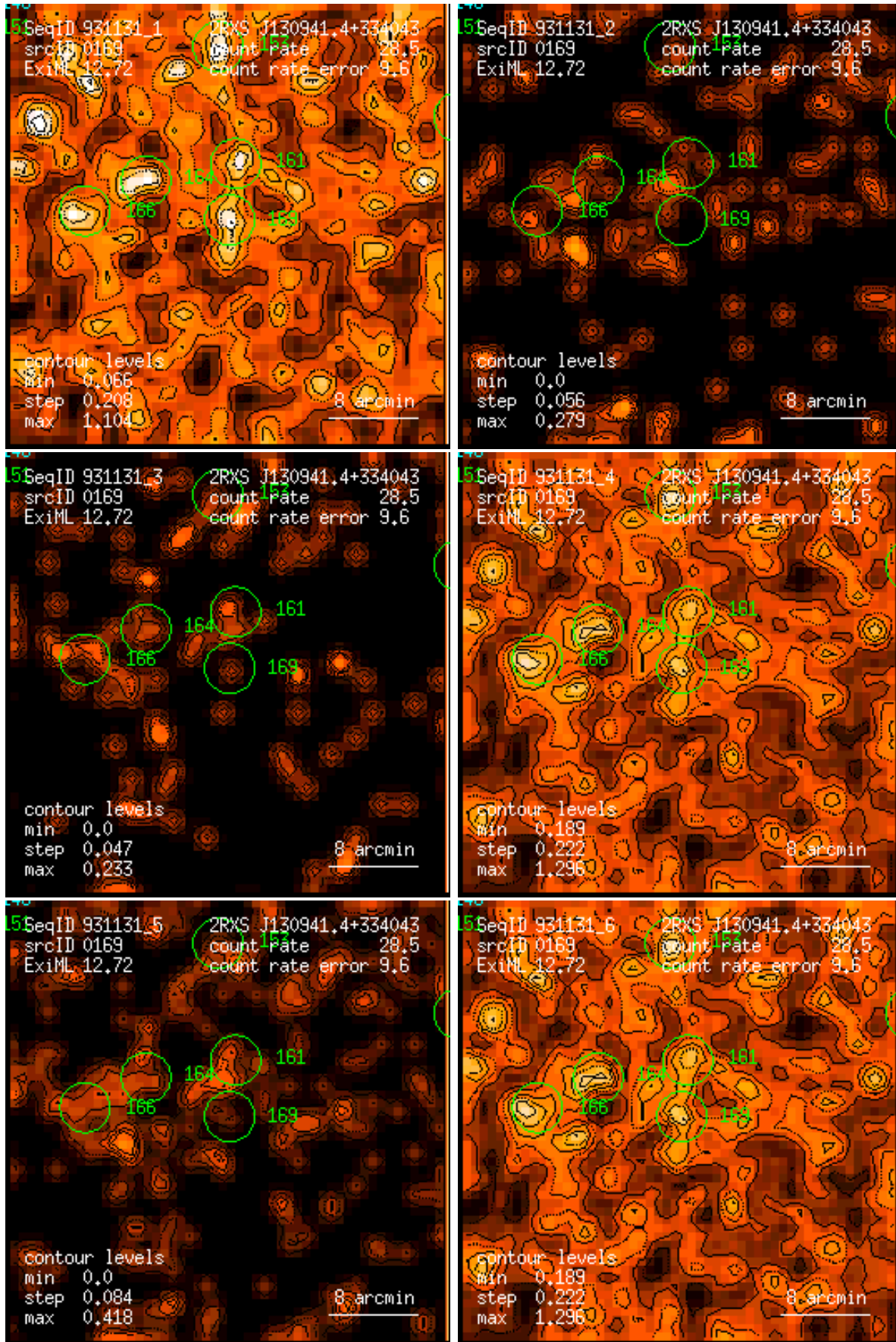
Figure 169: RASS 931131: detection 0169: band rate images, Gaussian filter: (1) PSPC channels 11 – 41, (2) 52 – 90, (3) 91 – 201, (4) 11 – 235, (5) 52 – 201, (6) 11 – 201. Broad band rates in counts/ks. Band rate contour levels in counts/ks/arcmin 2 .
