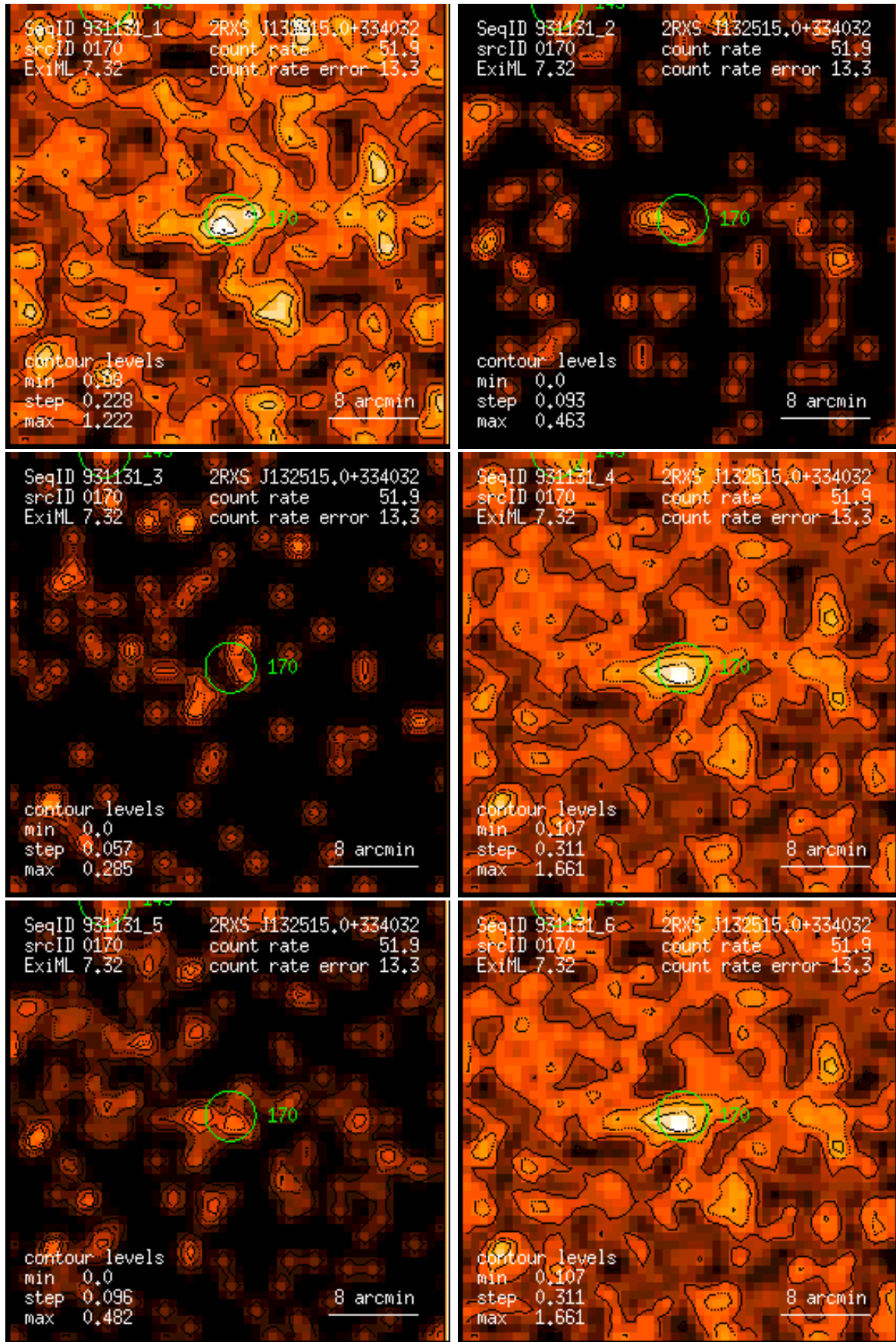
Figure 170: RASS 931131: detection 0170: band rate images, Gaussian filter: (1) PSPC channels 11 – 41, (2) 52 – 90, (3) 91 – 201, (4) 11 – 235, (5) 52 – 201, (6) 11 – 201. Broad band rates in counts/ks. Band rate contour levels in counts/ks/arcmin 2 .
