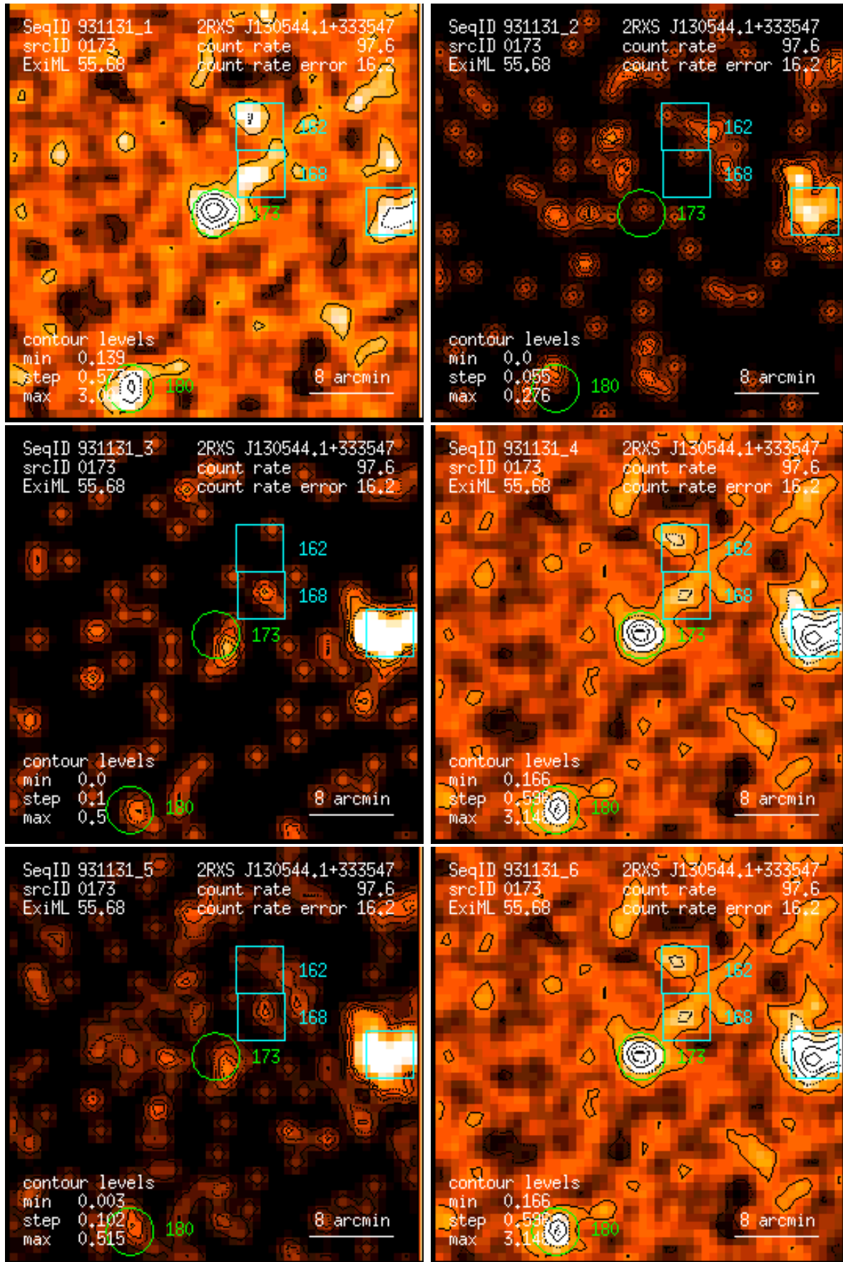
Figure 173: RASS 931131: detection 0173: band rate images, Gaussian filter: (1) PSPC channels 11 – 41, (2) 52 – 90, (3) 91 – 201, (4) 11 – 235, (5) 52 – 201, (6) 11 – 201. Broad band rates in counts/ks. Band rate contour levels in counts/ks/arcmin 2 .
