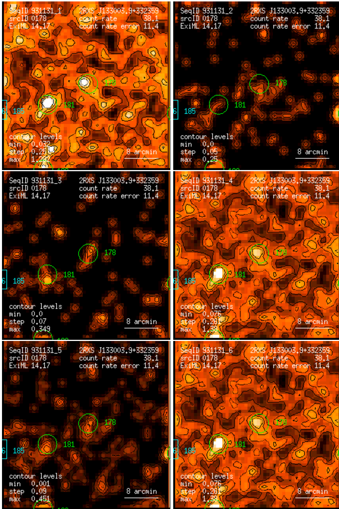
Figure 178: RASS 931131: detection 0178: band rate images, Gaussian filter: (1) PSPC channels 11 – 41, (2) 52 – 90, (3) 91 – 201, (4) 11 – 235, (5) 52 – 201, (6) 11 – 201. Broad band rates in counts/ks. Band rate contour levels in counts/ks/arcmin 2 .
