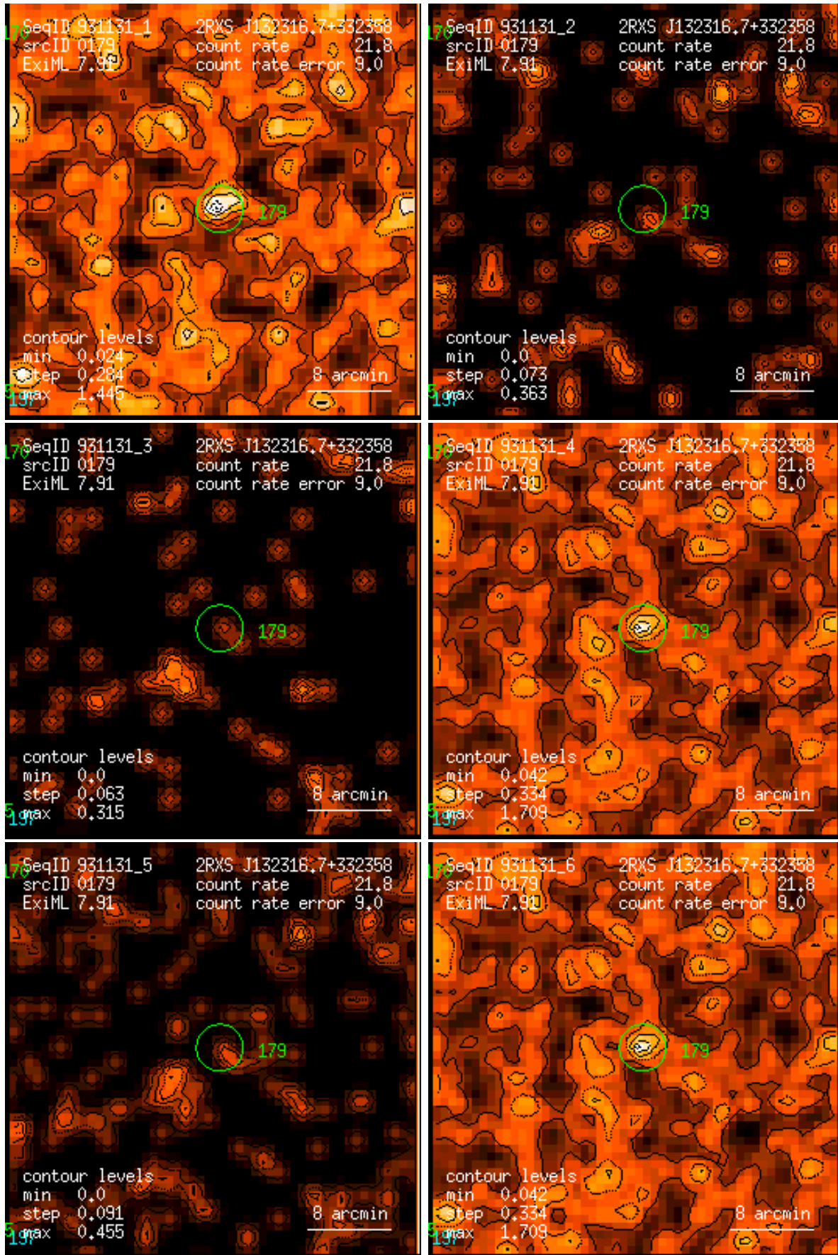
Figure 179: RASS 931131: detection 0179: band rate images, Gaussian filter: (1) PSPC channels 11 – 41, (2) 52 – 90, (3) 91 – 201, (4) 11 – 235, (5) 52 – 201, (6) 11 – 201. Broad band rates in counts/ks. Band rate contour levels in counts/ks/arcmin 2 .
