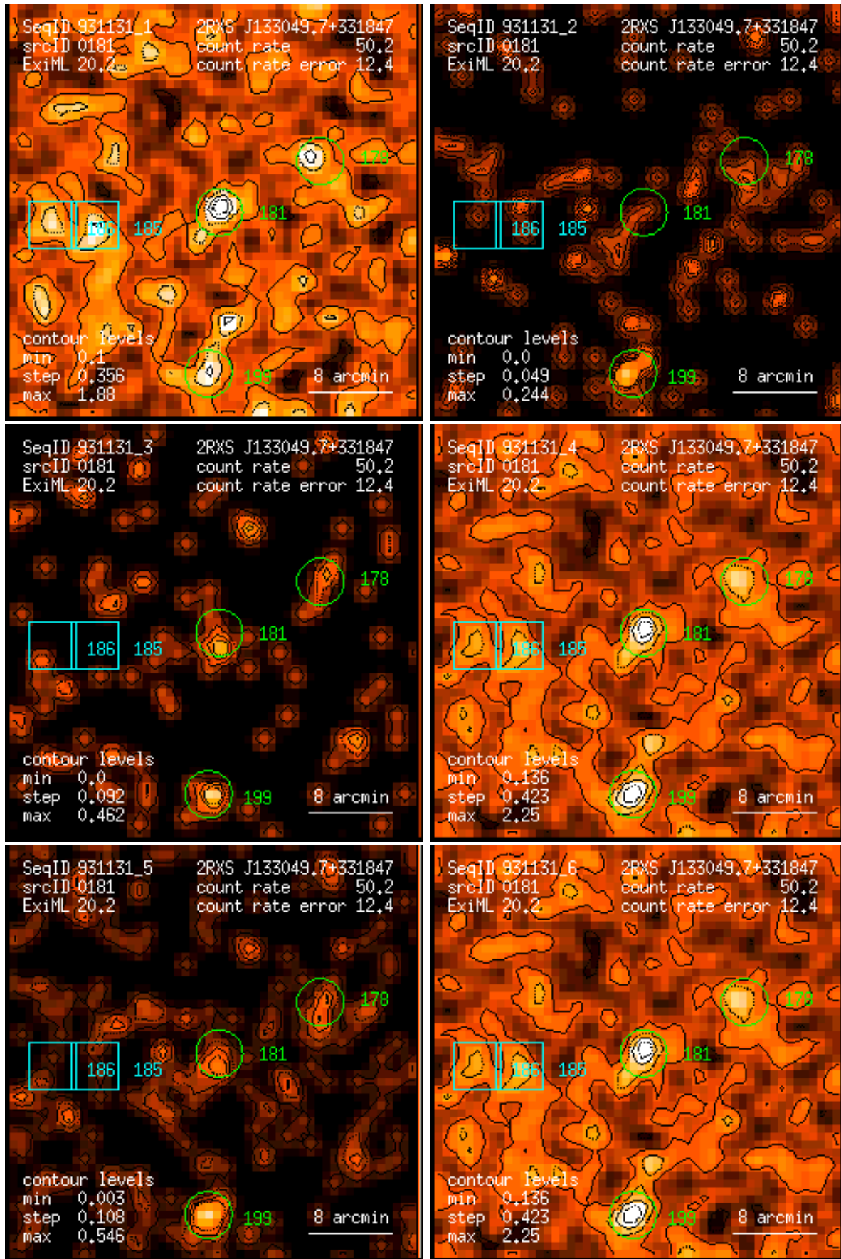
Figure 181: RASS 931131: detection 0181: band rate images, Gaussian filter: (1) PSPC channels 11 – 41, (2) 52 – 90, (3) 91 – 201, (4) 11 – 235, (5) 52 – 201, (6) 11 – 201. Broad band rates in counts/ks. Band rate contour levels in counts/ks/arcmin 2 .
