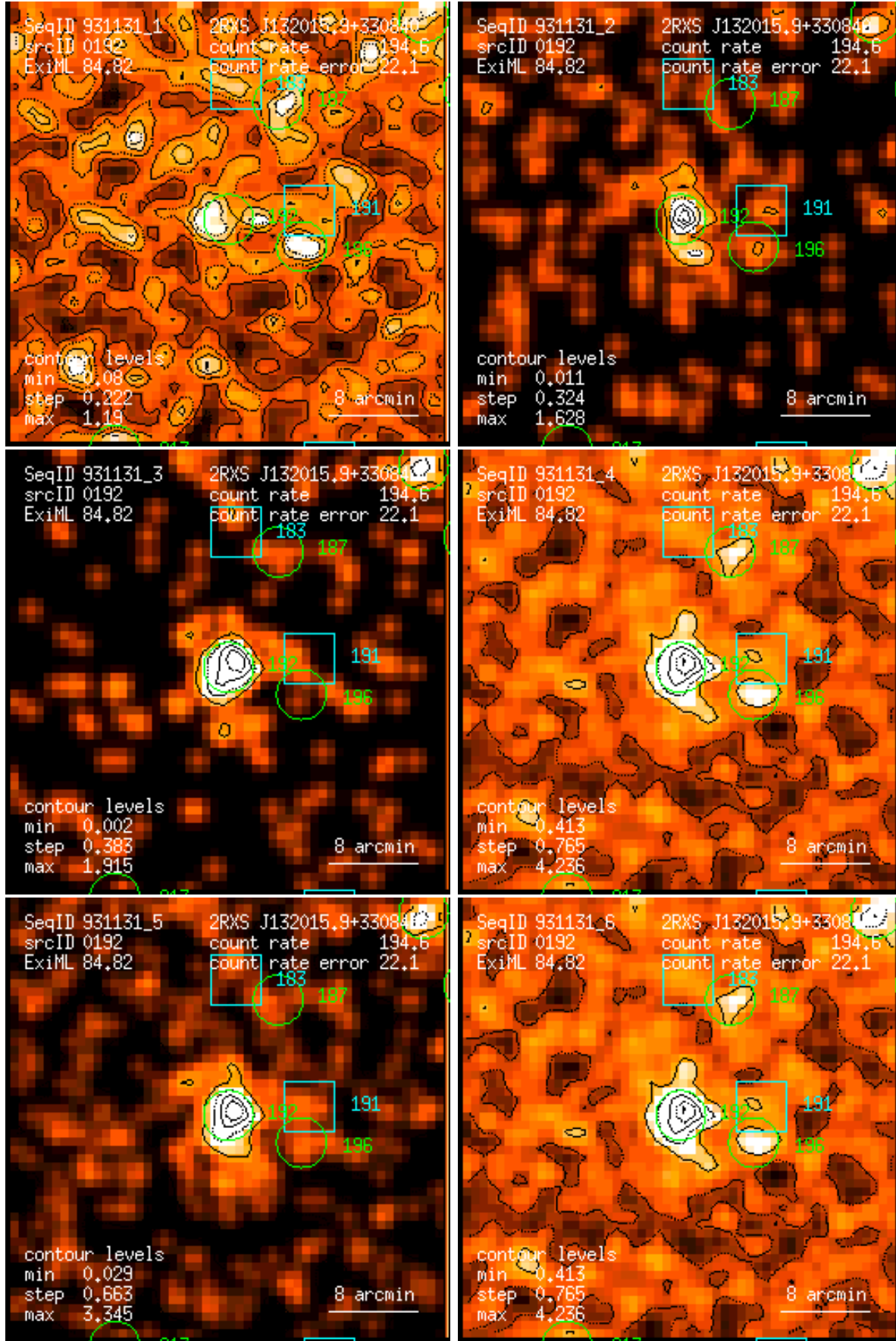
Figure 192: RASS 931131: detection 0192: band rate images, Gaussian filter: (1) PSPC channels 11 – 41, (2) 52 – 90, (3) 91 – 201, (4) 11 – 235, (5) 52 – 201, (6) 11 – 201. Broad band rates in counts/ks. Band rate contour levels in counts/ks/arcmin 2 .
