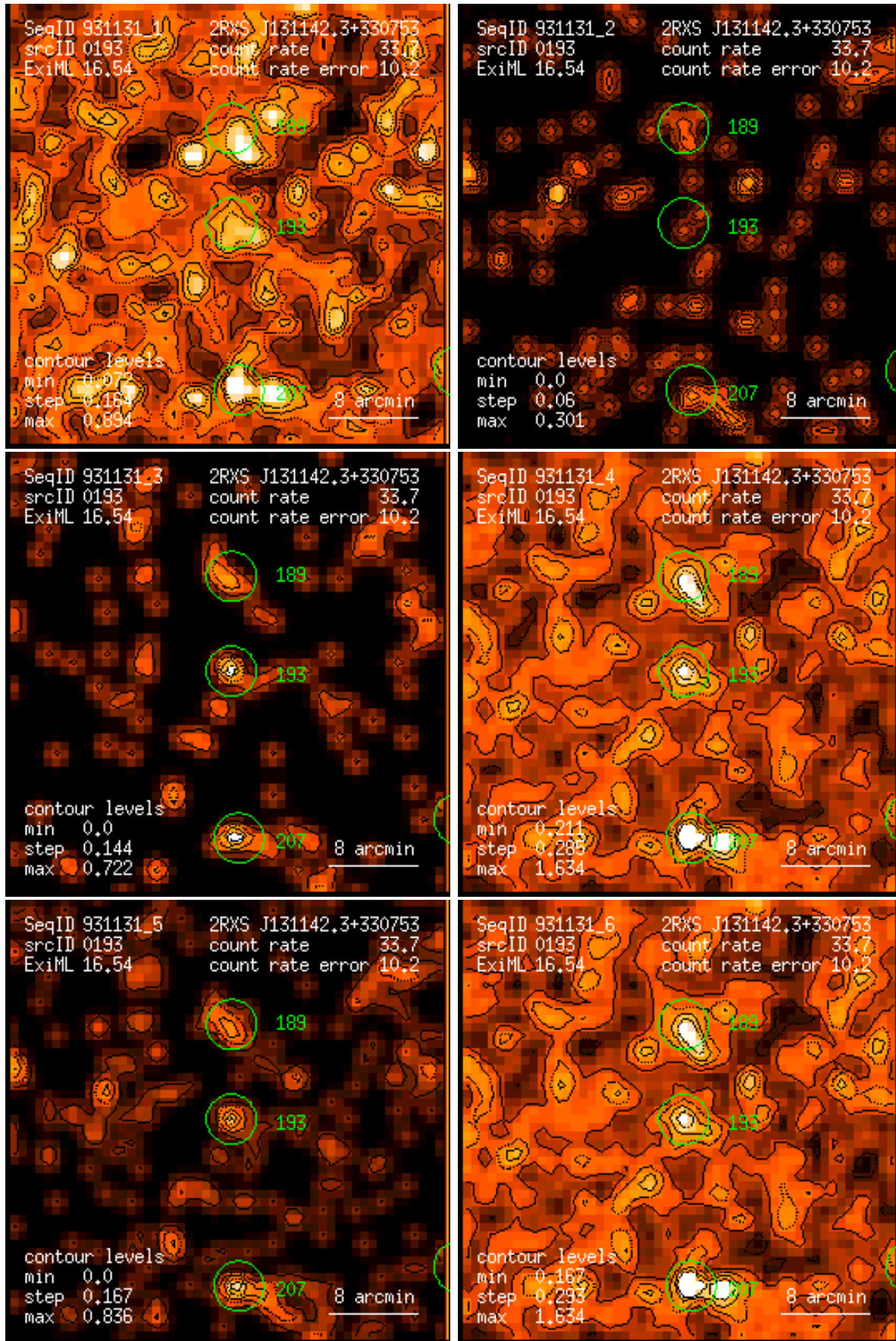
Figure 193: RASS 931131: detection 0193: band rate images, Gaussian filter: (1) PSPC channels 11 – 41, (2) 52 – 90, (3) 91 – 201, (4) 11 – 235, (5) 52 – 201, (6) 11 – 201. Broad band rates in counts/ks. Band rate contour levels in counts/ks/arcmin 2 .
