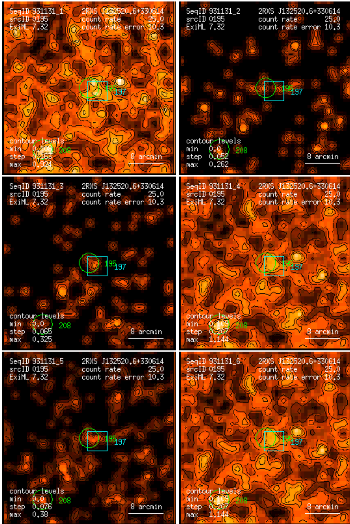
Figure 195: RASS 931131: detection 0195: band rate images, Gaussian filter: (1) PSPC channels 11 – 41, (2) 52 – 90, (3) 91 – 201, (4) 11 – 235, (5) 52 – 201, (6) 11 – 201. Broad band rates in counts/ks. Band rate contour levels in counts/ks/arcmin 2 .
