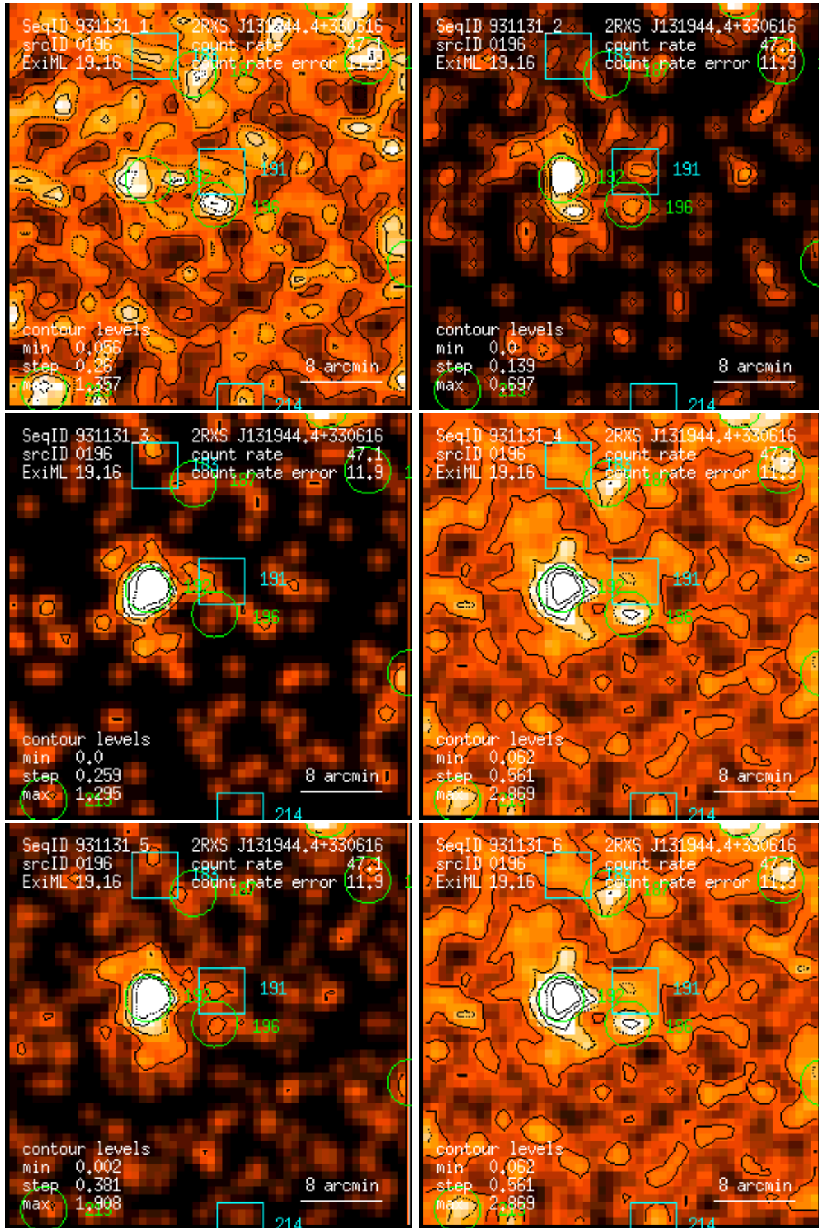
Figure 196: RASS 931131: detection 0196: band rate images, Gaussian filter: (1) PSPC channels 11 – 41, (2) 52 – 90, (3) 91 – 201, (4) 11 – 235, (5) 52 – 201, (6) 11 – 201. Broad band rates in counts/ks. Band rate contour levels in counts/ks/arcmin 2 .
