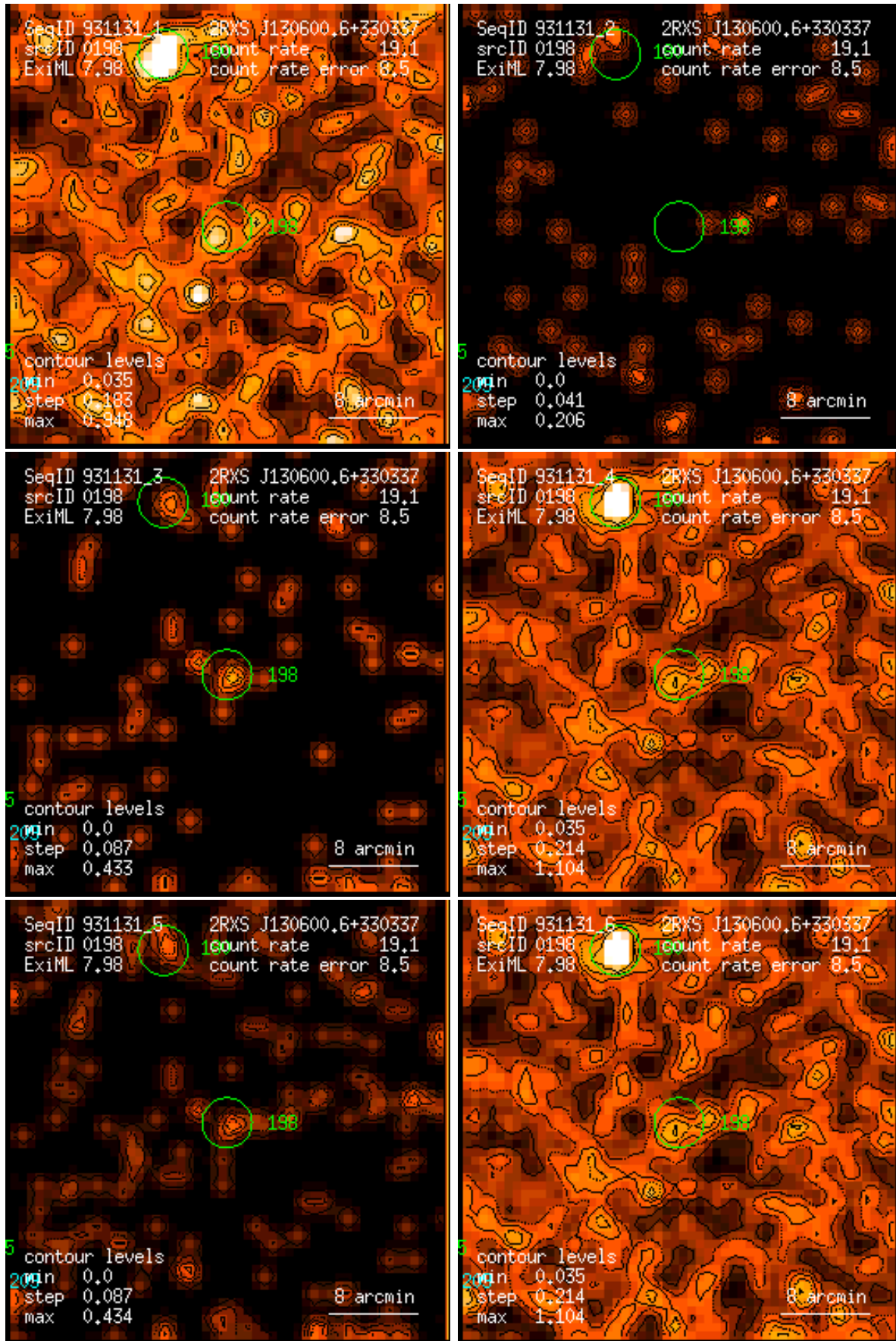
Figure 198: RASS 931131: detection 0198: band rate images, Gaussian filter: (1) PSPC channels 11 – 41, (2) 52 – 90, (3) 91 – 201, (4) 11 – 235, (5) 52 – 201, (6) 11 – 201. Broad band rates in counts/ks. Band rate contour levels in counts/ks/arcmin 2 .
