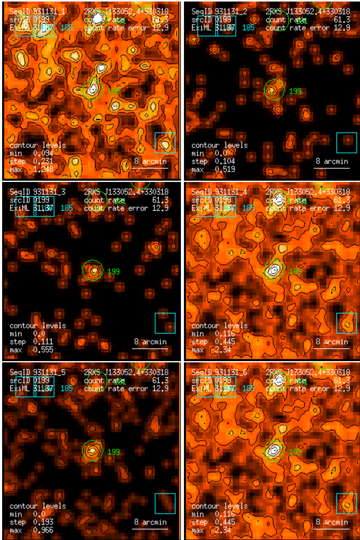
Figure 199: RASS 931131: detection 0199: band rate images, Gaussian filter: (1) PSPC channels 11 – 41, (2) 52 – 90, (3) 91 – 201, (4) 11 – 235, (5) 52 – 201, (6) 11 – 201. Broad band rates in counts/ks. Band rate contour levels in counts/ks/arcmin 2 .
