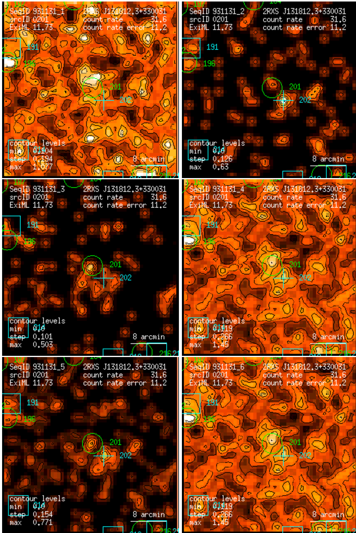
Figure 201: RASS 931131: detection 0201: band rate images, Gaussian filter: (1) PSPC channels 11 – 41, (2) 52 – 90, (3) 91 – 201, (4) 11 – 235, (5) 52 – 201, (6) 11 – 201. Broad band rates in counts/ks. Band rate contour levels in counts/ks/arcmin 2 .
