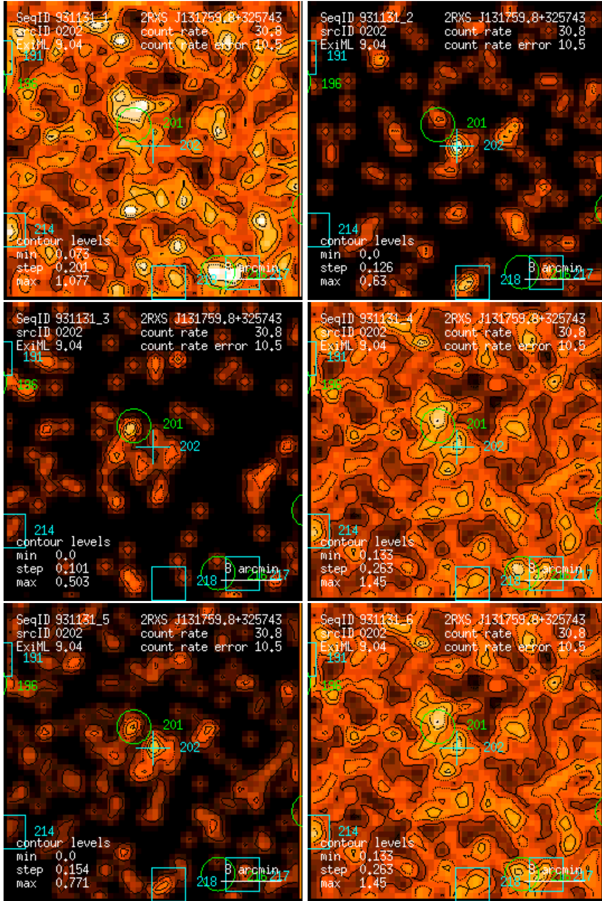
Figure 202: RASS 931131: detection 0202: band rate images, Gaussian filter: (1) PSPC channels 11 – 41, (2) 52 – 90, (3) 91 – 201, (4) 11 – 235, (5) 52 – 201, (6) 11 – 201. Broad band rates in counts/ks. Band rate contour levels in counts/ks/arcmin 2 .
