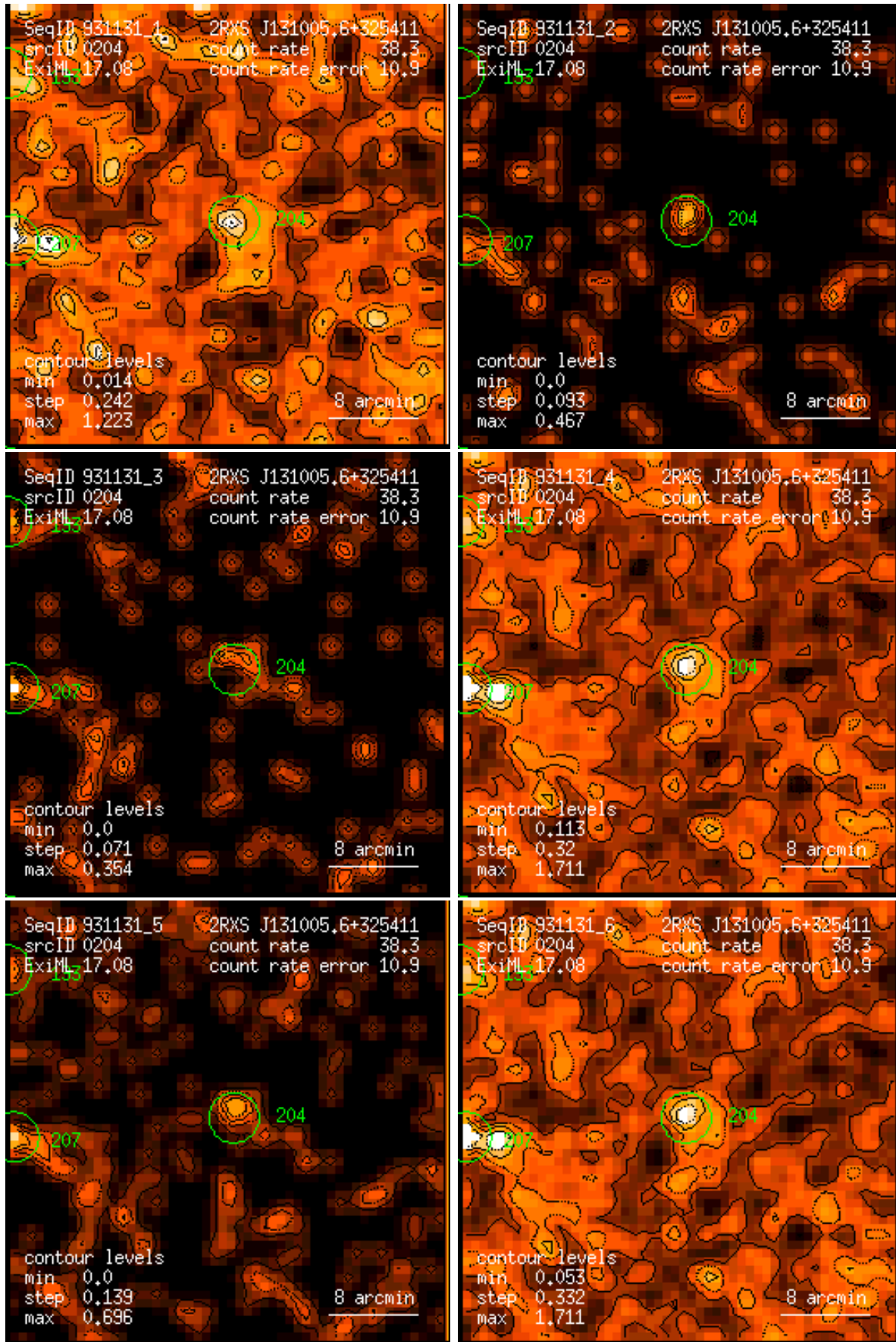
Figure 204: RASS 931131: detection 0204: band rate images, Gaussian filter: (1) PSPC channels 11 – 41, (2) 52 – 90, (3) 91 – 201, (4) 11 – 235, (5) 52 – 201, (6) 11 – 201. Broad band rates in counts/ks. Band rate contour levels in counts/ks/arcmin 2 .
