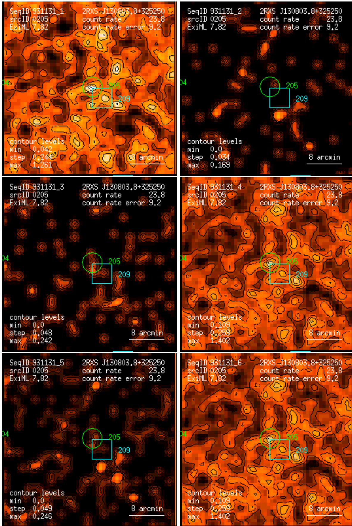
Figure 205: RASS 931131: detection 0205: band rate images, Gaussian filter: (1) PSPC channels 11 – 41, (2) 52 – 90, (3) 91 – 201, (4) 11 – 235, (5) 52 – 201, (6) 11 – 201. Broad band rates in counts/ks. Band rate contour levels in counts/ks/arcmin 2 .
